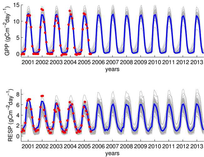
Figure 11. DALECV2 monthly estimates for GPP and RESP at Morgan Monroe State forest. The red dots are the observations, the blue trajectories are obtained using the 4DVAR analysis, the gray -grey trajectories are ensemble runs obtained from a 95% confidence sample of the posterior pdf.
