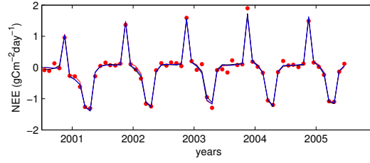
Figure 5. Solution of the linearized-linearised inverse problem for NEE. The red points represent the observations, the red curve is the true trajectory, the green curve is the trajectory obtained using the unstable solution and the blue curve is obtained using the TSVD solution.
