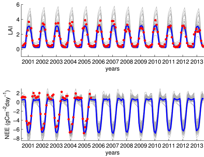
Figure 10. DALECV2 monthly estimates for LAI and NEE at Morgan Monroe State forest. The red dots are the observations, the blue trajectories are obtained using the 4DVAR analysis, the gray -grey trajectories are ensemble runs obtained from a 95% confidence sample of the posterior pdf.
