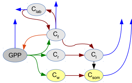
Figure 1. DALECV2 links the carbon pools (C) via allocation fluxes (green), litterfall fluxes (red), decomposition decomposition (black). Respiration is represented by the blue arrows. The orange arrow represents the feedback of foliar carbon to gross primary production (GPP).
