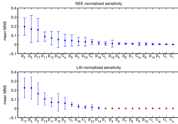
Figure 2. Mean normalized normalised sensitivities : 100 parameter sets satisfying EDCs are sampled at the Morgan Monroe State Forest. Parameters are ranked in decreasing order according to their sensitivity, the blue dots represent the mean of the MNS (dimensionless quantity) and the intervals represent 1-sigma error bars; the red dots correspond to null sensitivity.
