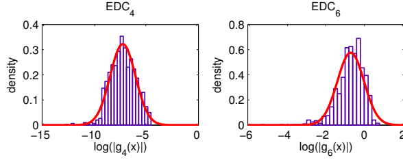
Figure 3. distribution and gaussian -Gaussian fit for EDC 4 and EDC 6 .
