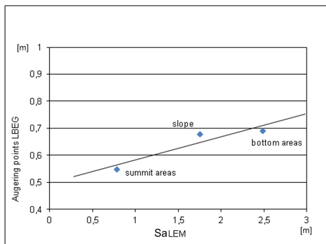
Figure 13 The average regolith thickness values [m] of the drilling points compared to the average values of the SaLEM model run within the units of the geomorphographical map of the validation rectangle.
