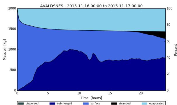
Figure 4. Plot of the time evolution of the oil budget of a 24 hour simulation with OpenOil. Of 2000 kg oil initially at the ocean surface, more than 20% is seen to evaporate within the first few hours. The amount of oil submerged due to wave action and ocean turbulence varies with the wind and wave conditions, with more oil resurfacing when wind decreases after about 8 hours. After about 18 hours, some of the oil seen to hit the coastline. These results are for the oiltype "AVALDSNES", very different results could be obtained if using another oiltype for the same geophysical conditions.
