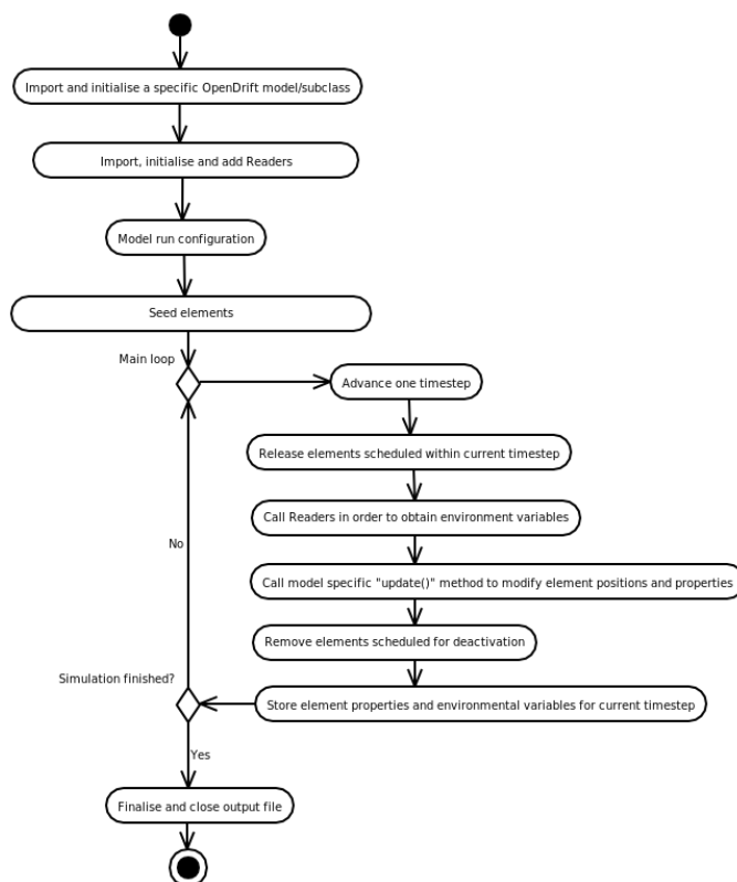
Figure 1. Flowchart of an OpenDrift simulation.
