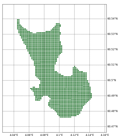
Figure 3. Oil drift simulation initialised by seeding 2000 oil elements within contours of an oil slick as observed from satellite (Radarsat2). The contour is imported from a GML file produced by Kongsberg Satellite Services (KSAT).
