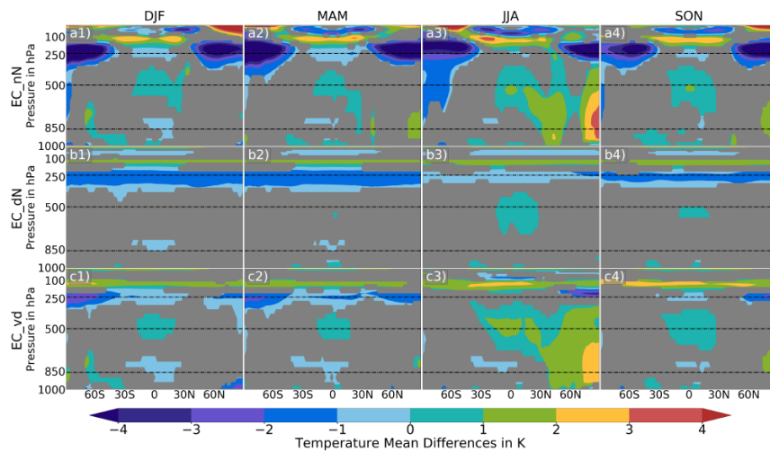
Figure 6.1: Vertical profile of the zonal averaged seasonal differences of temperature climatology to ERA-Interim. Plots show differences between the model simulations EC_{nN} (a), EC_{dN} (b), EC_{vd} (c) and ERA-Interim over the boreal winter (DJF, 1), spring (MAM, 2), summer (JJA, 3) and autumn (SON, 4) according to the two sided Welch-test. Differences between the two fields which are not statistically significant to the t test (95% confidence interval) are masked in gray. The dashed lines mark pressure levels 250hPa, 500hPa and 850hPa and are provided later on a global perspective.
