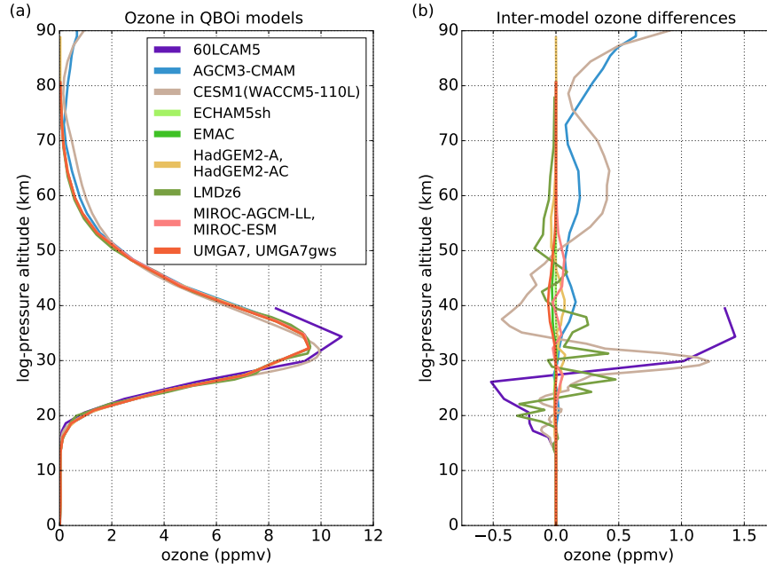
Figure 6. (a) Vertical profiles in the tropics of the climatological ozone concentration prescribed in QBOi timeslice experiments (Experiments 2–4; Table 5 indicates which models have performed these experiments), for models that do not include ozone chemistry (as indicated in Table 8) and excluding MPI-ESM-MR and UMGC2 which uploaded existing hindcast data for Experiment 5a. Each vertical profile is an average over the 5°S–5°N latitude band, zonal mean, and annual mean. (b) As (a), but showing differences from a reference profile so that inter-model variations are more clearly visible. The reference profile is the 1988–2007 climatology of the SPARC ozone referred to in Appendix A (item A1; under item A2, ). The period 1988–2007 is the SST and sea ice climatological period same as that recommended for Experiment 2 for the SST and sea ice climatologies (Appendix A, item A2).
