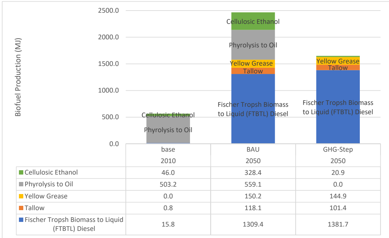
46 47 Figure S8: CA-TIMES' biofuel production by biofuel and scenario.
