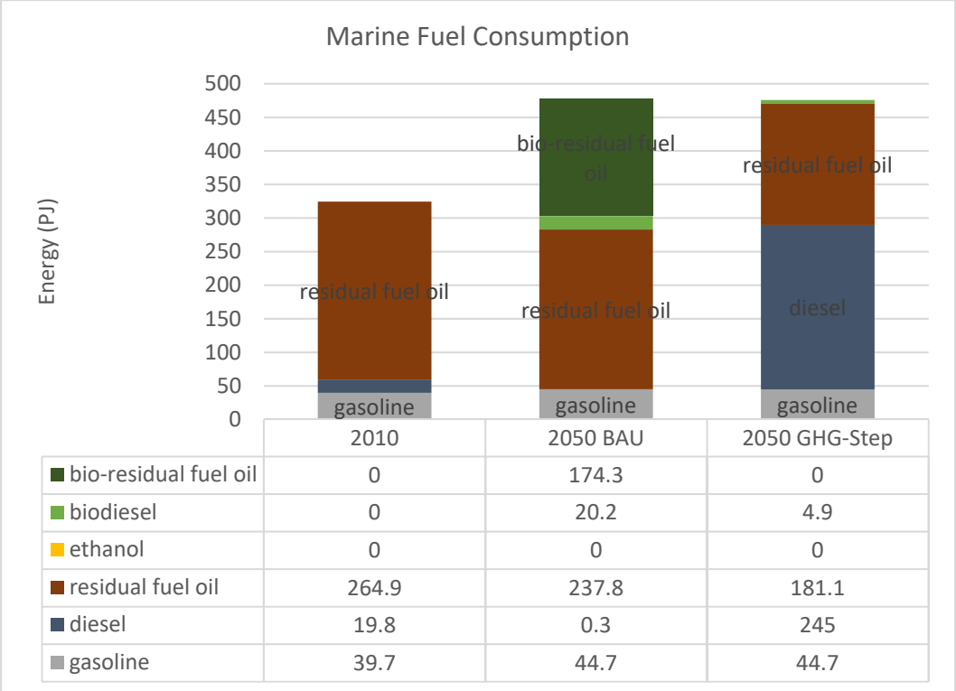
Figure S4: CA-TIMES' fuel consumption by fuel type and scenario for marine.
