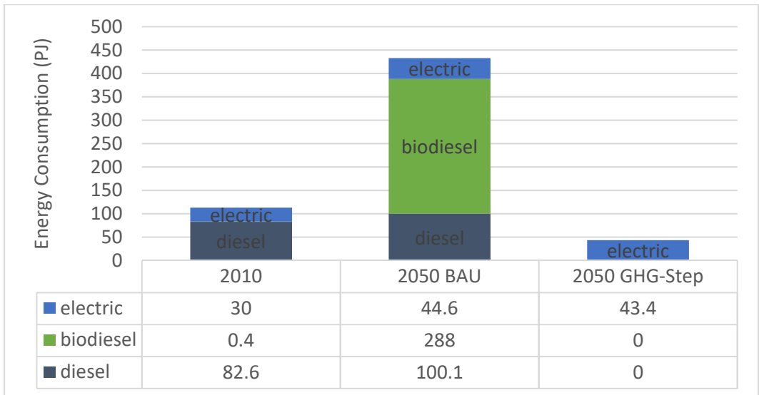
15 Figure S1: CA-TIMES' energy consumption by fuel type and scenario for rail.
