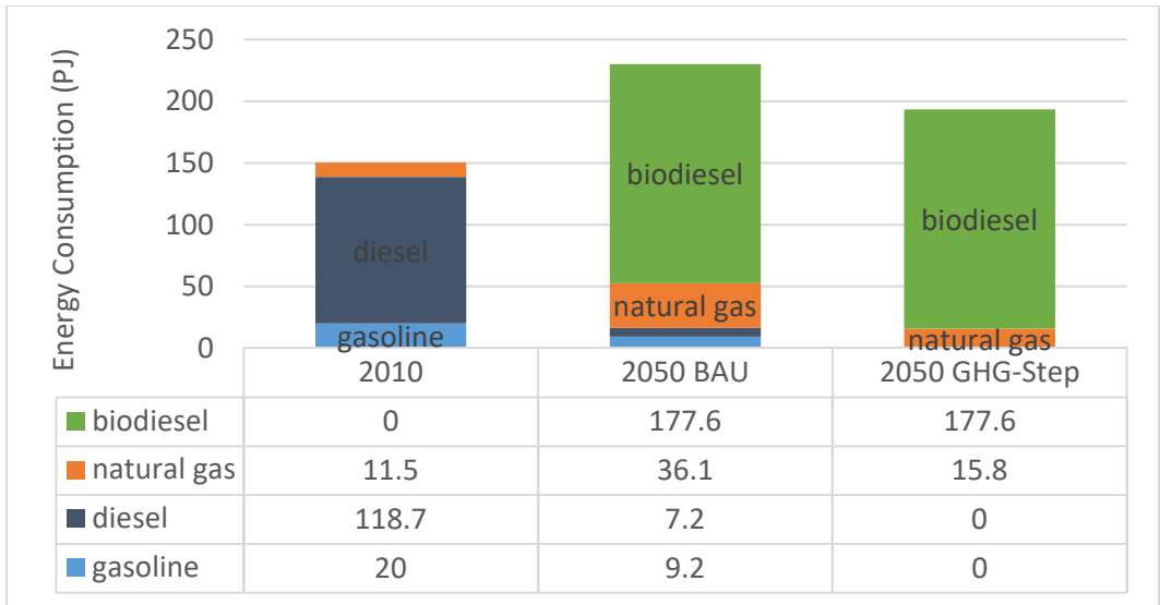
18 19 Figure S2: CA-TIMES Energy consumption by fuel type and scenario for off-road vehicles.
