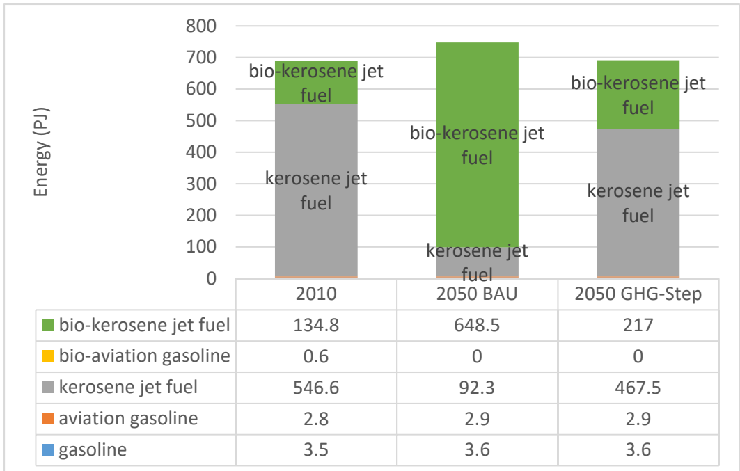
21 22 Figure S3: CA-TIMES' energy consumption by fuel type and scenario for aircraft.
