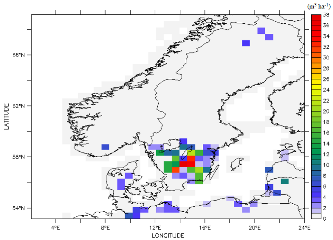
Figure 8. Simulated spatial distribution of the damaged wood volume ( m^3 ha^{-1} ) over southern Sweden by Gudrun in January 2005.
