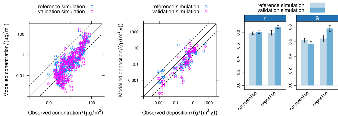
Figure 15. Comparison of modelled and observed dust concentration and deposition: scatterplots of monthly concentrations (left) and annual deposition (centre), and barcharts of the corresponding correlation coefficients r and skill scores S (right). The observations are taken from the AEROCOM dust benchmark (Huneus et al., 2011).
