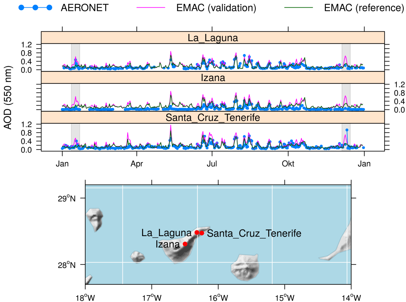
Figure 10. Time series of the daily mean AOD at the Canarian AERONET stations (top) and a map showing the location of the stations (bottom). The white squares depict the T106 model grid. During the grey shaded periods of the time series in January and December, at least one of the three AERONET stations observed an AOD peak which is reproduced by the validation but not by the reference simulation.
