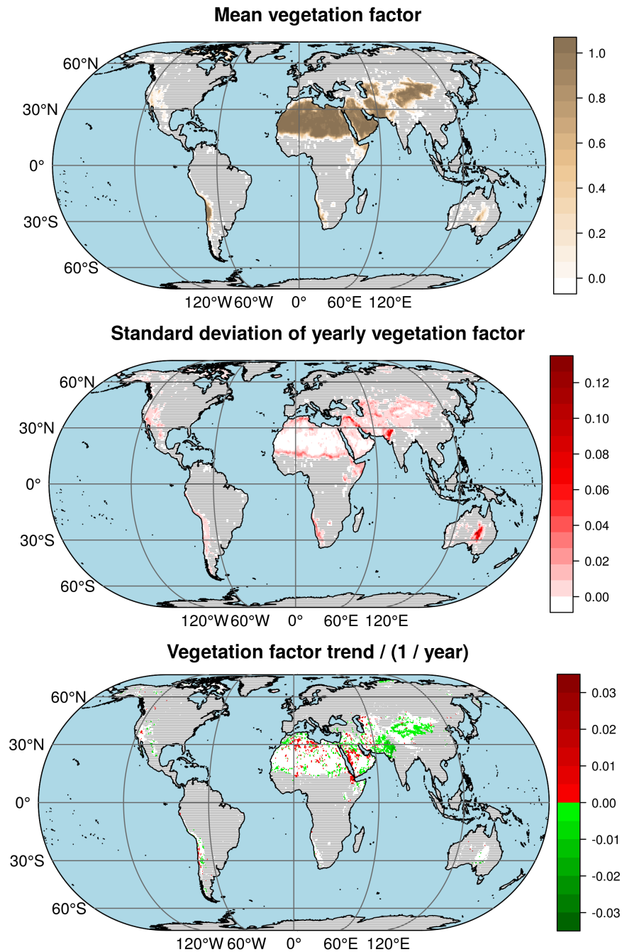
Figure 2. Vegetation factor based on leaf area index data from Yuan et al. (2011) averaged over the period 2000 to 2015 (top), the standard deviation of the annual mean values (center) and the trend of the annual mean values (bottom). Regions where the landcover mask precludes emissions throughout the period of available landcover data (2001 to 2012) are hatched.
