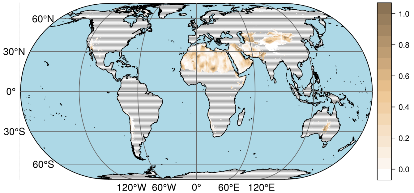
Figure 5. The topography factor defined by Eq. 3, calculated using the GMTED2010 elevation data. Regions where the landcover mask precludes emissions throughout the period of available landcover data (2001 to 2012) are hatched.
