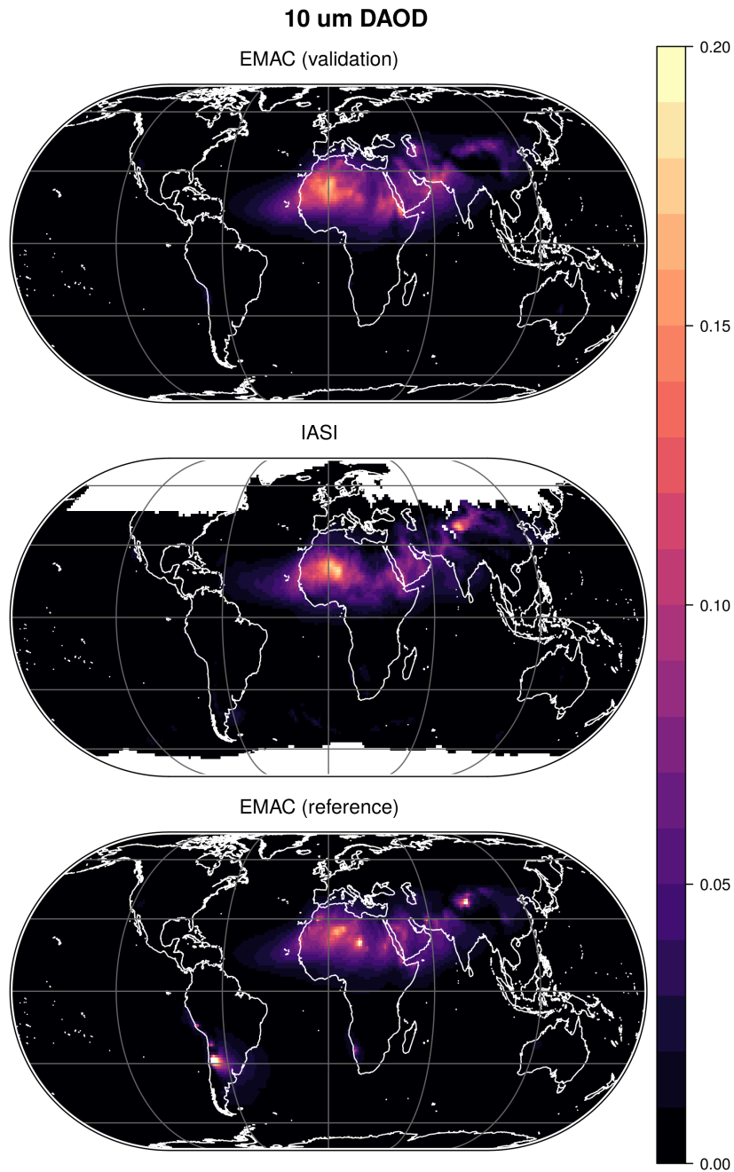
Figure 13. Annual mean for 2011 of the DAOD at 10 \mu\text{m} wavelength observed by IASI (centre) and simulated by EMAC with (“validation”, top) and without (“reference”, bottom) revision of the dust emission scheme. The revised dust emissions enhance the correlation of the AOD pattern from 0.79 to 0.89, the skill score from 0.64 to 0.78.
