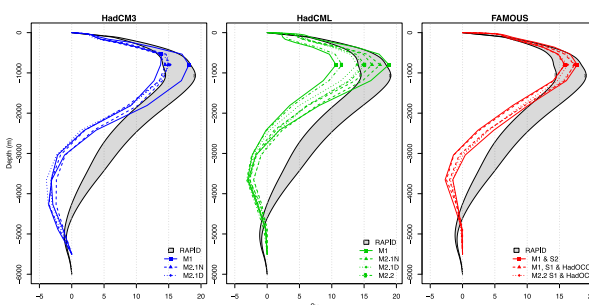
Figure 8. Annual depth profiles of the Atlantic meridional overturning circulation (AMOC) at 26.25^\circ \text{N} showing range of values for variants of HadCM3, HadCM3L and FAMOUS. Annual data from the RAPID array at 26.5^\circ \text{N} is highlighted in grey. The depth at which the AMOC reaches its maximum is indicated with a point.
