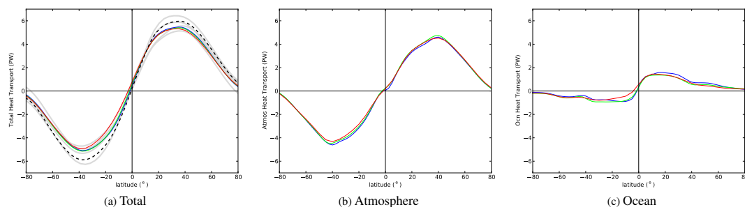
Figure 5. The annual mean northward heat transport in total, the atmosphere and the ocean. Black line shows the observational estimate, blue: HadCM3-M2.1, green: HadCM3L-M2.1 and red: FAMOUS-M2.2. These transports are calculated as the implied heat transports from the TOA and surface energy fluxes (see Trenberth and Fasullo (2013) for details). Observational estimates for the total transport are derived from the CERES data.
