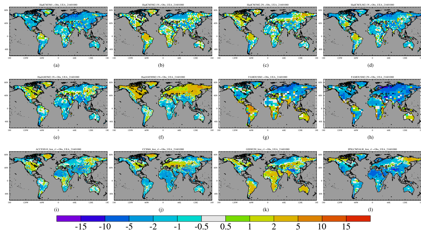
Figure 3. (a) The difference between the annual mean surface air temperature (in ^{\circ}\text{C} ) of our version of HadCM3-M1 and the CRU CL v2.0 for the period 1960–1990 regrided onto the HadCM3-M1 grid, (b) As (a) for the HadCM3-M2.1 version, (c) As (a) but for HadCM3-M2.2, (d) As (a) but for the HadCM3L-M2.1N version, (e) As (a) but for HadAM3-M2.1, (f) As (a) but for HadAM3H-M2.1, (g) As (a) but for FAMOUS-M1, and (h) As (a) but for FAMOUS-M2.2. (i), (j), (k) and (l) show comparable results for four CMIP5 models, ACCESS1-0, CCSM4, GISS-E2-H and IPSL-CM5A-LR respectively. These were chosen to represent two models which were above the CMIP5 average in terms of their RMSE with respect to surface air temperature, and two models which were below average. All differences are calculated by regriding the CRU data onto the corresponding model grid, using simple bi-linear interpolation.
