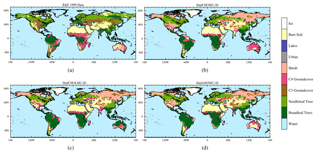
Figure 9. Maps of the dominant plant functional type for observations (a) and model simulations of the pre-industrial. The models shown are (b) HadCM3-M2.1D (c) HadCM3L-M2.1D and (d) HadAM3-M2.1D. The observed dataset for comparison is Ramankutty and Foley (1999).
