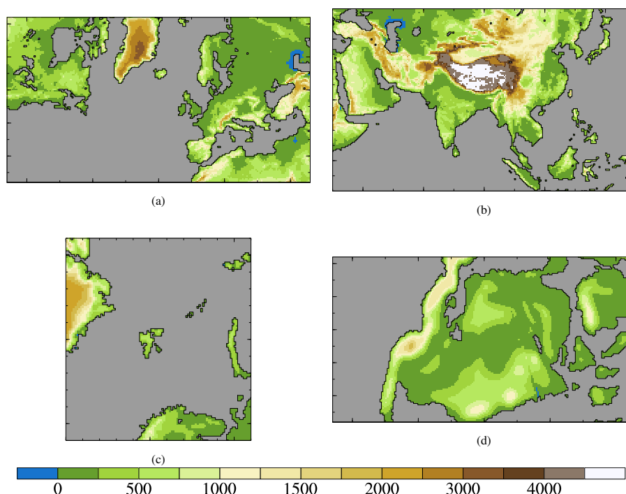
Figure 1. Land/sea mask and orography (sea coloured grey, land height in meters) for four configurations of HadRM3. (a) Shows the standard European domain at 0.44^\circ resolution, (b) shows the equivalent domain for E. Asia, (c) shows a configuration for the Arctic and Svalbard at 0.22^\circ (as used in Day et al., 2012), and (d) a N. America/European configuration for the early Cretaceous at 0.44^\circ resolution (as used in Haywood et al., 2004)
