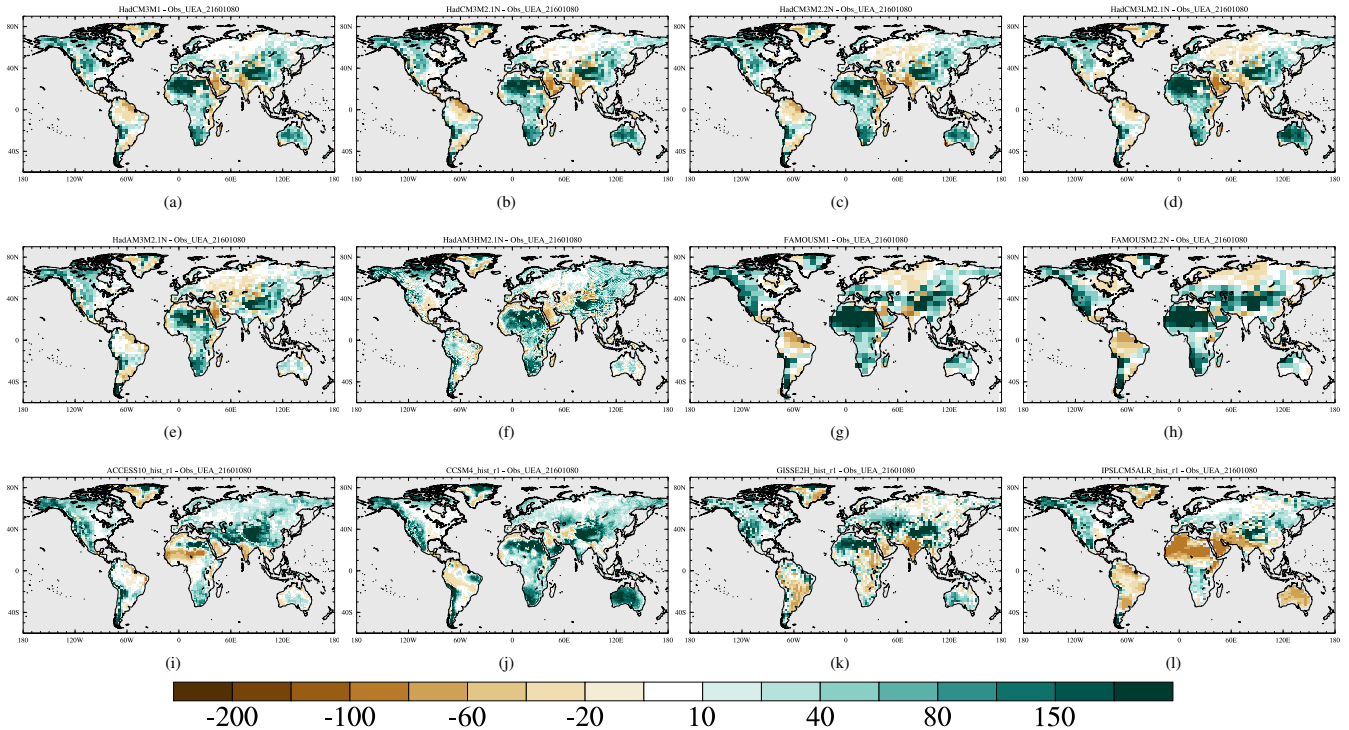
Figure 4. As for Fig.3 except showing the difference in mean annual precipitation, expressed as a % difference to the CRU CL v2.0 observations.
