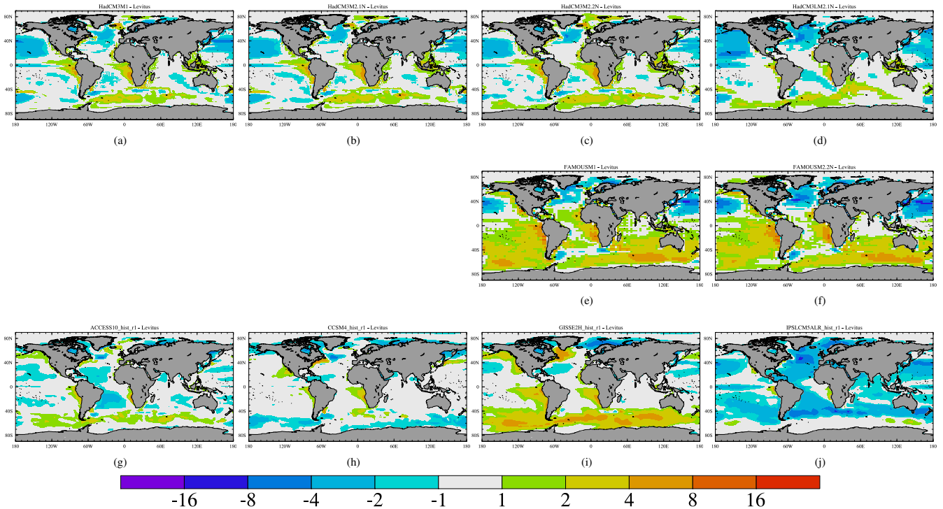
Figure 6. Annual mean sea surface temperature differences (in °C) for a range of coupled model simulations, and also for the same four CMIP5 models used in Figs. 3 and 4. The observational dataset is the Levitus World Ocean Atlas (2009) (Locarnini et al., 2010). The figure shows the difference in SST between model and observations for (a) HadCM3-M1, (b) HadCM3-M2.1, (c) HadCM3-M2.2, (d) HadCM3L-M2.1, (e) FAMOUS-M1, (f) FAMOUS-M2.2, (g) ACCESS1.0, (h) CCSM4, (i) GISS-E2-H, and (j) IPSL-CM5A-LR. Model output is regridded to the same resolution of the observations.
