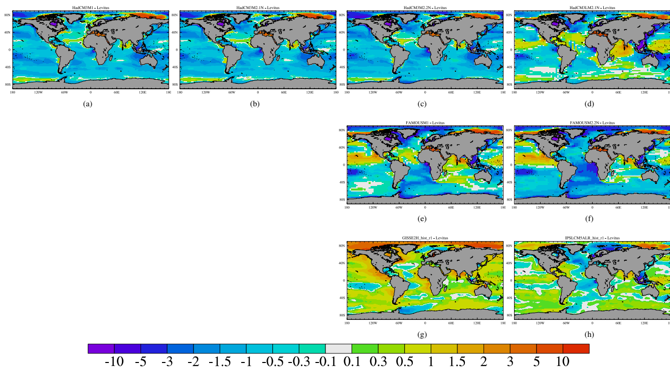
Figure 7. As Fig. 6 but showing the differences in sea surface salinity (in \text{g kg}^{-1} ) between models and observations. (a) HadCM3-M1, (b) HadCM3-M2.1, (c) HadCM3-M2.2, (d) HadCM3L-M2.1, (e) FAMOUS-M1, (f) FAMOUS-M2.2, (g) GISS-E2-H, and (h) IPSL-CM5A-LR. The observational dataset is the Levitus World Ocean Atlas (2009) (Antonov et al., 2010). Model output is regridded to the same resolution of the observations.
