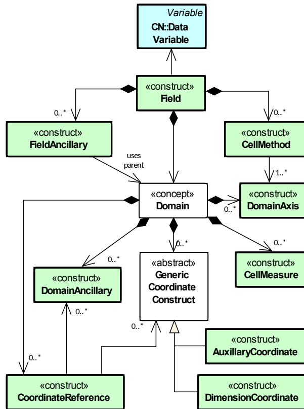
Figure 9. The nine constructs of the CF data model (corresponding to the green layer in figure 1) described using UML (appendix A). In this and all other CF data model diagrams, the CF data model constructs are labelled with the “construct” stereotype to distinguish them from other data model elements which appear in other diagrams as green boxes with no label. The field construct corresponds to a CF-netCDF data variable. Relationships between other constructs and CF-netCDF are given in figures 10 and 11. The domain provides the linkage between the field construct and the constructs which describe measurement locations and cell properties. It is not a construct of the data model (see section 4.1), but is an abstract concept that is useful for understanding the data model. Similarly, it is useful to define an abstract generic coordinate construct that can be used to refer to coordinates when their type (dimension or auxiliary coordinate construct) is not an issue.
