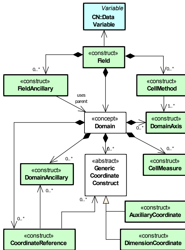
Figure 9. The nine constructs of the our CF data model (corresponding to the green layer in figure 1) described using UML (appendix A). In this and all other CF data model diagrams, the CF data model constructs are labelled with the “construct” stereotype to distinguish them from other data model elements which appear in other diagrams as green boxes with no label. The field construct corresponds to a CF-netCDF data variable. Relationships between other constructs and CF-netCDF are given in figures 10 and 11. The domain provides the linkage between the field construct and the constructs which describe measurement locations and cell properties. It is not a construct of the data model (see section 4.1), but is an abstract concept that is useful for understanding the data model it . Similarly, it is useful to define an abstract generic coordinate construct that can be used to refer to coordinates when their type (dimension or auxiliary coordinate construct) is not an issue.
