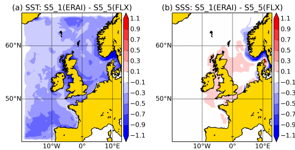
Figure 15. Comparison of mean SST (a) and SSS (b) differences between ERAI fluxes and NWP fluxes (S5_1 Vs S5_5).
