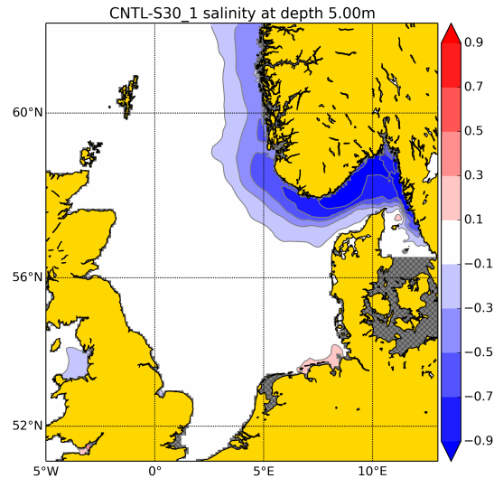
Figure 11. Comparison of mean salinity at 5 m between CO5 with 51 vertical levels using the Siddorn and Furner stretching function (CNTL) and 33 vertical levels using the Song and Haidvogel stretching function (S30_1).
