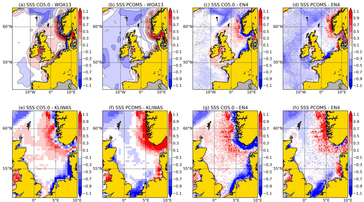
Figure 6. Mean model Sea Surface Salinity (SSS) differences 1985-2004 from WOA13, KLIWAS and EN4. (a) CO5 - WOA13 Climatology. (b) POLCOMS - WOA13 Climatology. (c) CO5 - EN4 (d) POLCOMS - EN4. (e) CO5 - KLIWAS North Sea Climatology. (f) POLCOMS - KLIWAS North Sea Climatology. (g) CO5 - EN4 in the North Sea. (h) POLCOMS - EN4 the North Sea.
