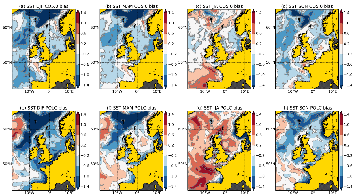
Figure 5. The difference between the mean seasonal model SST and the mean satellite SST for 1985-2004. (a) CO5 December-January-February (DJF) bias, (b) CO5 spring March-April-Mam (MAM) bias, (c) CO5 summer June-July-August (JJA) bias, (d) CO5 autumn bias September-October-November (SON), (e) POLCOMS (POLC) winter (DJF) bias, (f) POLC spring (MAM) bias, (g) POLC summer (JJA) bias, (h) POLC autumn bias (SON).
