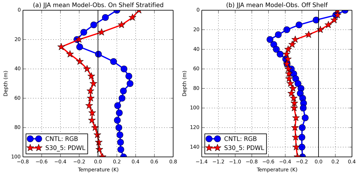
Figure 13. Comparison of summer time profiles compared to NEMO's three band light attenuation scheme (RGB) and POLCOMS 1 band scheme (PDWL). Panel (a) compares CNTL and S30_5 against the mean of profiles in the seasonally stratified part of the domain on shelf. Panel (b) compares CNTL and S30_5 against the mean of profiles off shelf south of 60° N.
