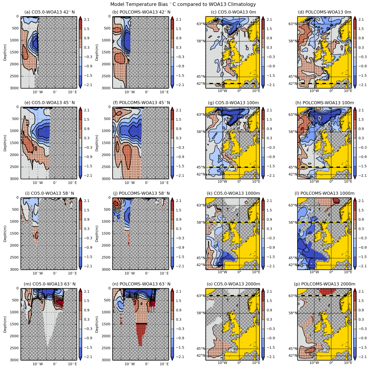
Figure 7. CO5 and POLCOMS temperature bias compared to WOA13 1985-2005. Panels (a), (e), (i) and (m) are CO5-WOA13 temperature bias transects along 42° N, 45° N, 58° N, and 63° N. Panels (b), (f), (j) and (n) are POLCOMS-WOA13 temperature bias transects along 42° N, 45° N, 58° N, and 63° N. Panels (c), (g), (k) and (o) are the CO5-WOA13 temperature bias at depths 0 m, 100 m, 1000 m and 2000 m. Panels (d), (h), (l) and (p) are the POLCOMS-WOA13 temperature bias at depths 0 m, 100 m, 1000 m and 2000 m.
