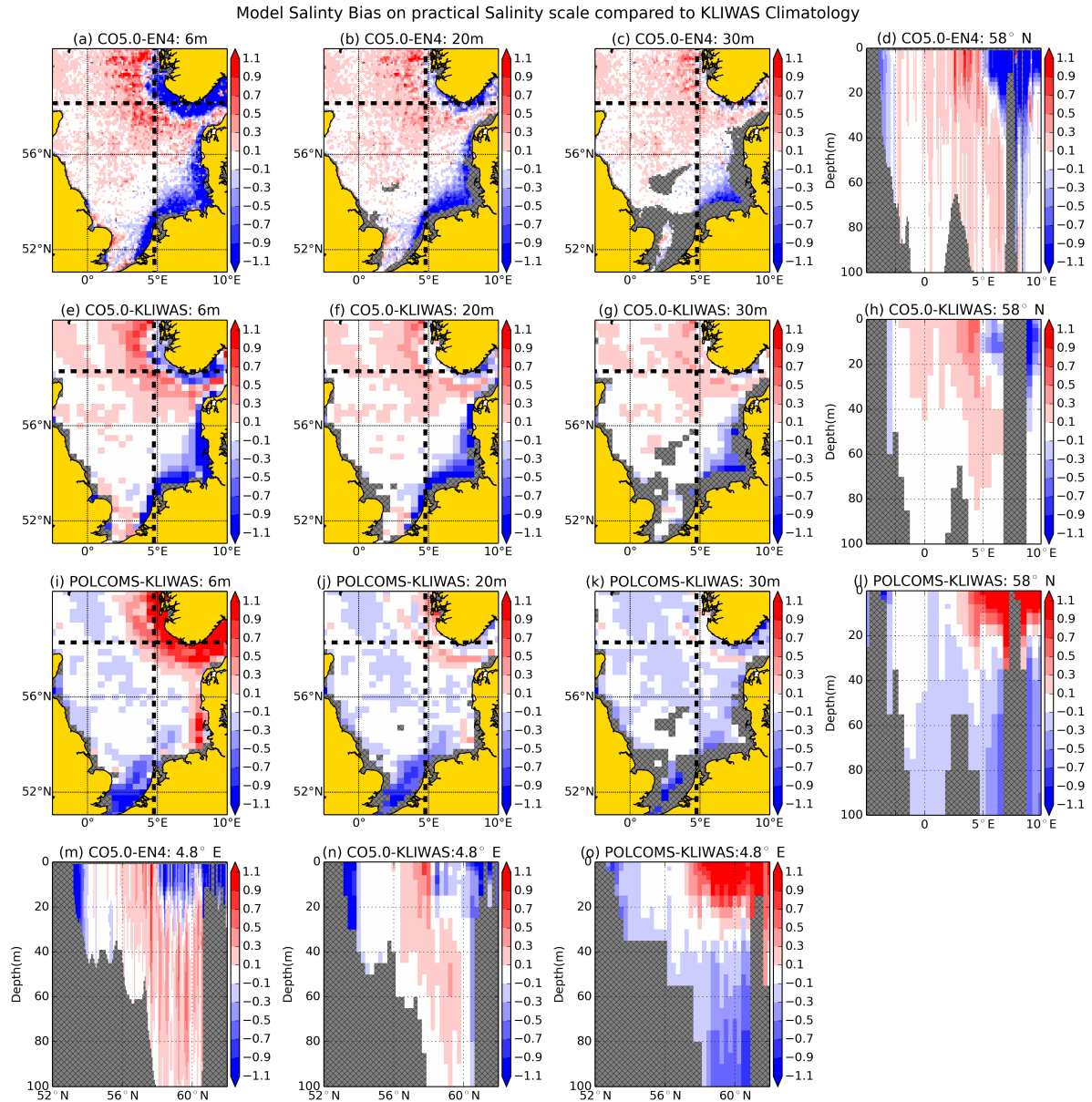
Figure 10. North Sea salinity bias compared to annual EN4 and KLIWAS climatology . Panels (a) - (d) compare CO5 and EN4 at 6 m, 20 m, 30 m and along a transect at 58° N. Panels (e) - (h) compare CO5 and KLIWAS climatology at 6 m, 20 m, 30 m and along a transect at 58° N. Panels (i) - (l) compare POLCOMS and KLIWAS climatology at 6 m, 20 m, 30 m and along a transect at 58° N. Panels (m) - (o) are transects through depth for each case along longitude 4.8° E.
