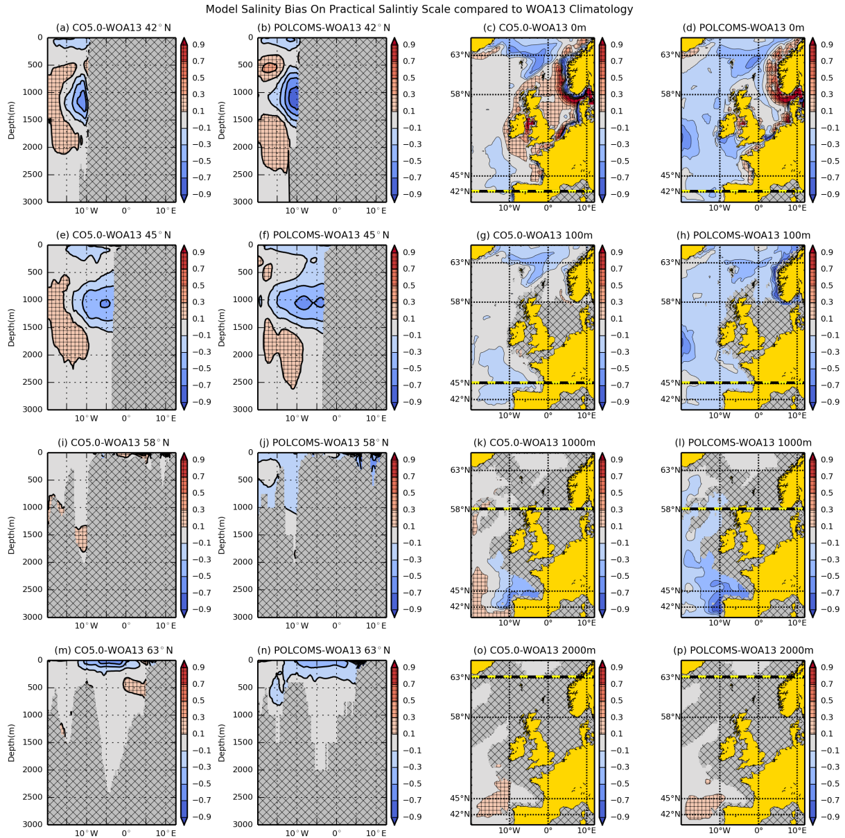
Figure 8. CO5 and POLCOMS salinity bias compared to WOA13 1985-2005. Panels (a), (e), (i) and (m) are CO5-WOA13 salinity bias transects along 42° N, 45° N, 58° N, and 63° N. Panels (b), (f), (j) and (n) are POLCOMS-WOA13 salinity bias transects along 42° N, 45° N, 58° N, and 63° N. Panels (c), (g), (k) and (o) are the CO5-WOA13 salinity bias at depths 0 m, 100 m, 1000 m and 2000 m. Panels (d), (h), (l) and (p) are the POLCOMS-WOA13 salinity bias at depths 0 m, 100 m, 1000 m and 2000 m.
