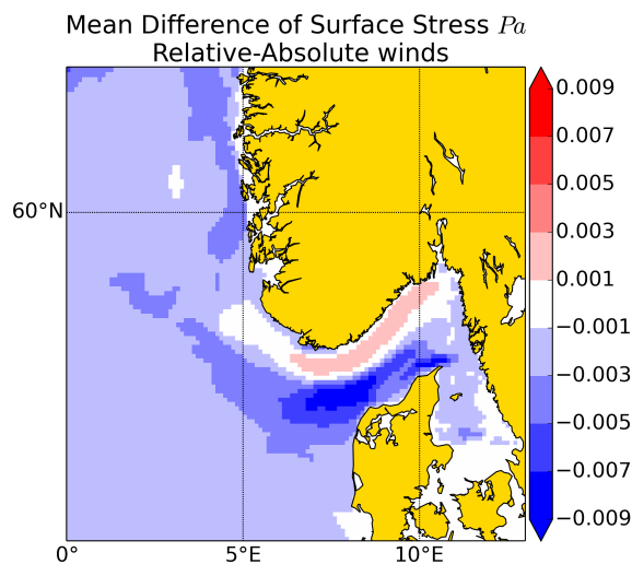
Figure 16. Comparison of mean surface shear stress in Pa between using wind velocity relative to ocean surface and absolute wind velocity.
