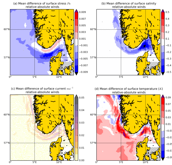
Figure 19. Comparison of mean surface shear stress in-between using wind velocity relative to ocean surface and absolute wind velocity for 2011 annual mean. Panel (a) Difference in surface shear stress in Pa. Panel (b) Difference in surface salinity Panel (c) Difference in surface current Panel (d) Difference in surface temperature
