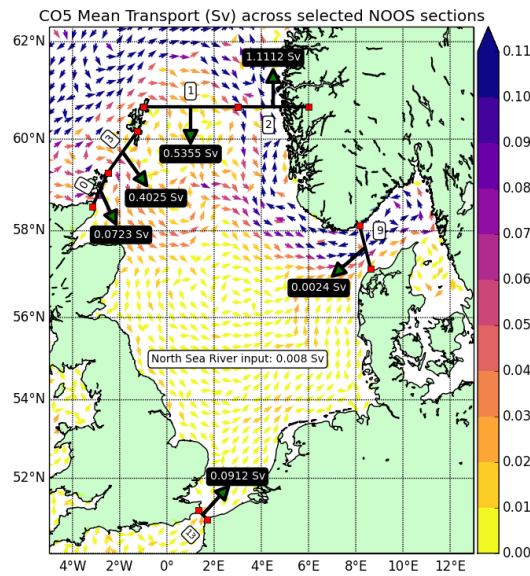
Figure 14. CO5 mean transport across selected NOOS transects surrounding the North Sea and the CO5 transport field shown only every 4th grid point for clarity.
