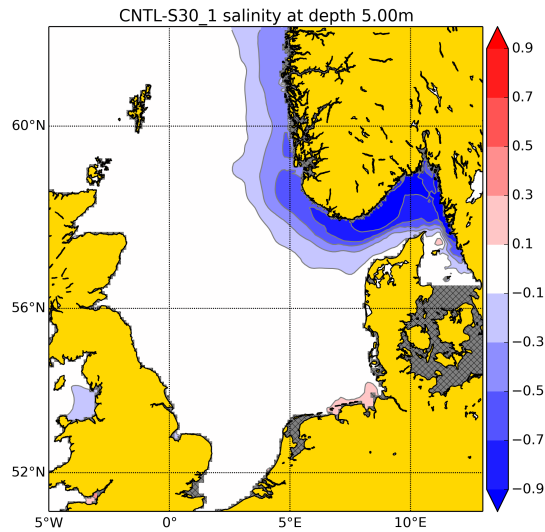
Figure 12. Comparison of mean salinity at 5 m between CO5 with 51 vertical levels using the Siddorn and Furner stretching function (CNTL) and 33 vertical levels using the Song and Haidvogel stretching function (S30_1). The hashed area in the Kattegat indicates the interface to Baltic NSBS model data.
