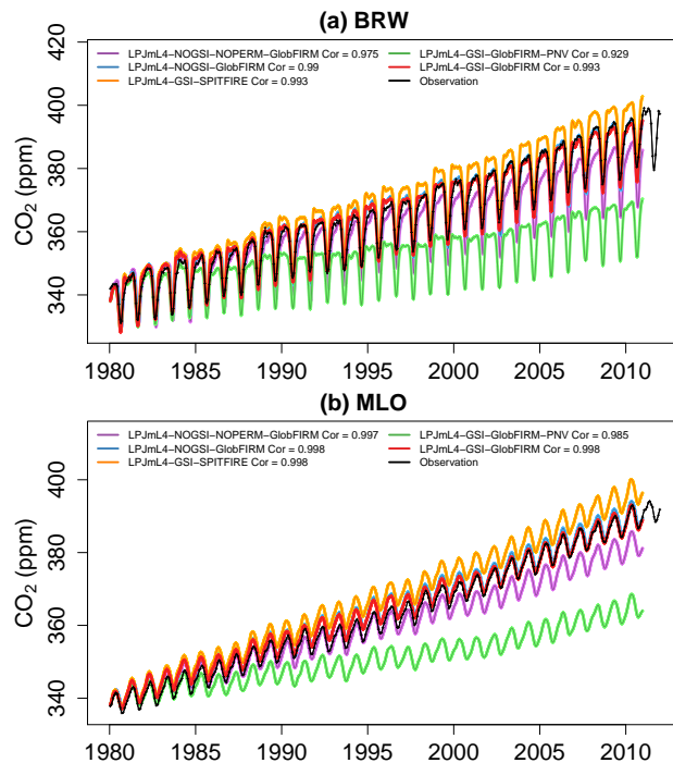
Figure 1. Comparison of the atmospheric CO 2 concentrations at Point Barrow (BRW) at the top and Mauna Loa (MLO) at the bottom for the different LPJmL4 experiments.
