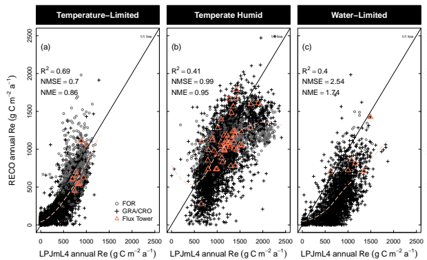
Figure 6. Ecosystem respiration ( R_e ) evaluation of standard LPJmL4 simulations with satellite-derived estimations from (Jägermeyr et al., 2014). Compared are annual R_e sums for all pixels from the displayed extent in SI-Fig. S70, separated by climate type (a)–(c). Dashed lines indicate a polynomial bias curve. Chart symbols are separated for forest (FOR) and grassland/cropland (GRA/CRO) land cover classes.
