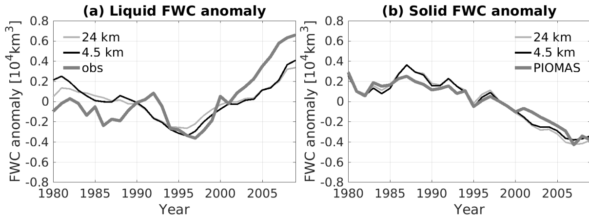
Figure 12. Anomalies of (a) liquid freshwater (FW) content and (b) solid FW content of the Arctic Ocean. The FW content is calculated using a reference salinity of 34.8. The liquid FW content observation is provided by Polyakov et al. (2013a) , and the solid FW content is compared to the data derived from PIOMAS reanalysis ( Schweiger et al., 2011 ).
