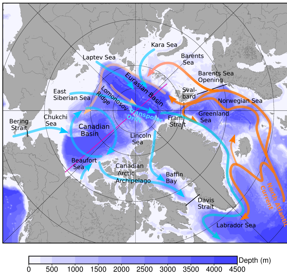
Figure 1. Schematic of main ocean circulations in the pan-Arctic Ocean. The freshwater circulation is shown with light blue curves, and the Atlantic Water (AW) circulation is shown with orange curves. The color patch in the background shows the ocean bottom bathymetry. The black lines indicate the four Arctic gateways. The magenta line crossing the North Pole indicates the location of the transect shown in Fig. 8e,f.
