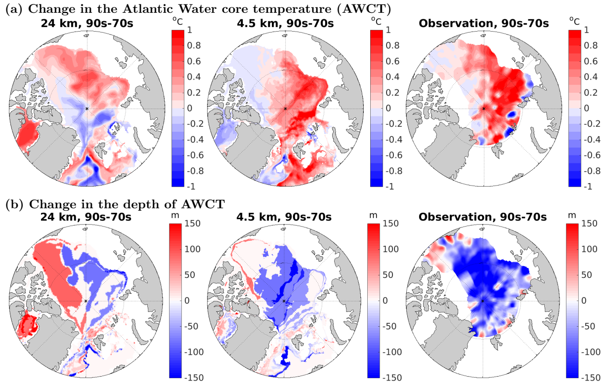
Figure 6. (a) Difference of the Atlantic Water core temperature (AWCT) between the 1990s mean and 1970s mean (the former minus the latter) in simulations (from left to right) LOW and HIGH and in observation ( Polyakov et al., 2012 ). (b) The same as (a) but for the depth of the AWCT. For the model results the shelf regions (<200 m) are not shown.
