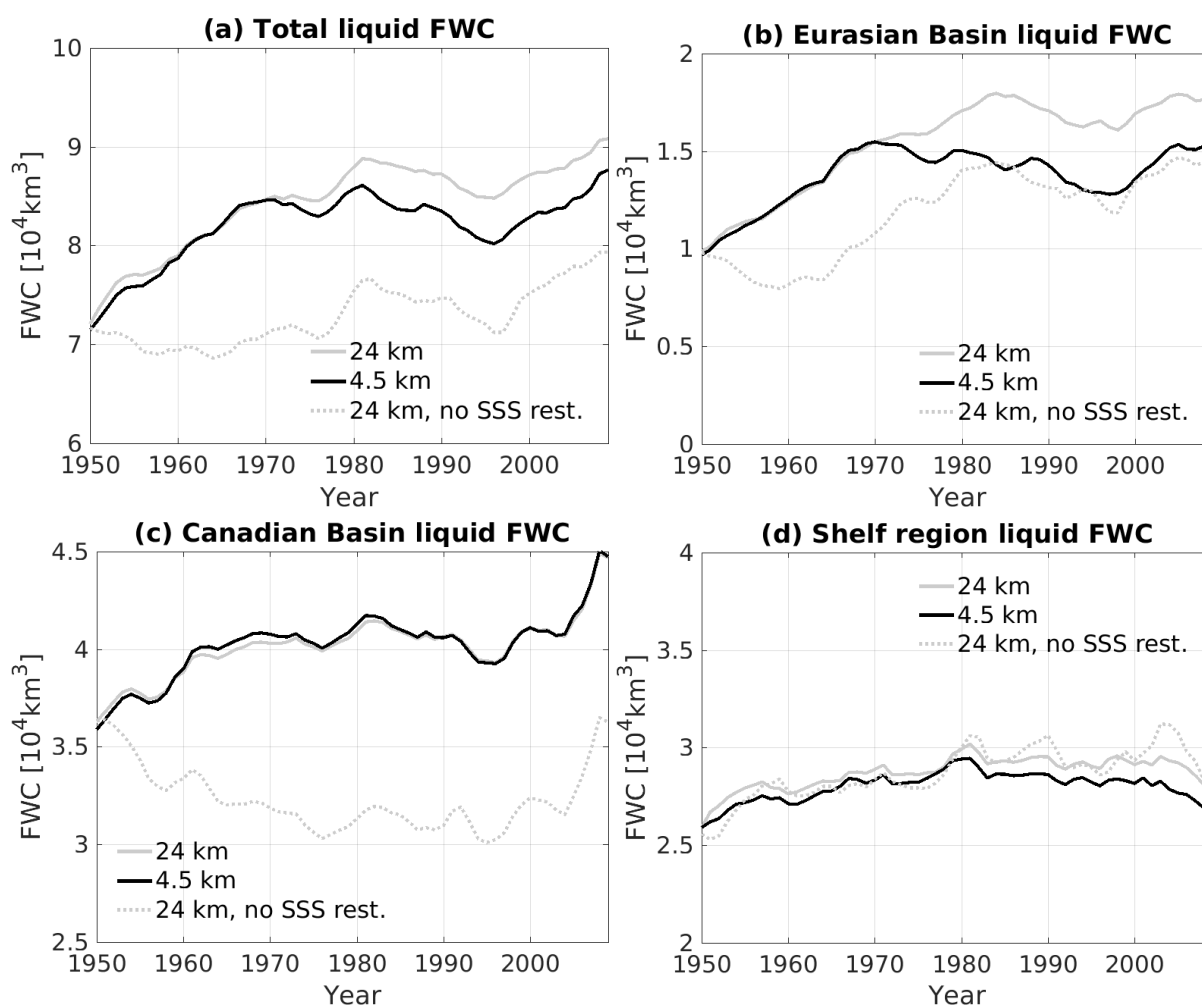
Figure 9. (a) The time series of annual mean total Arctic liquid freshwater (FW) content. The liquid FW content in Eurasian Basin, Canadian Basin and shelf regions are shown in (b)(c)(d), respectively. The FW content is calculated using a reference salinity of 34.8.
