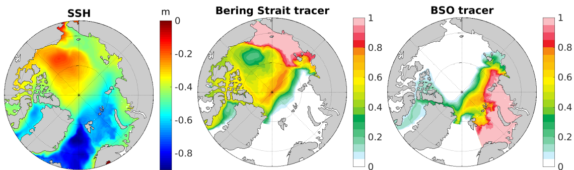
Figure 11. (a) Mean sea surface height (left), Bering Strait passive tracer (middle), and Barents Sea Opening (BSO) passive tracer (right) in simulation LOW for the period of 1993–2002. (b) The same as (a) but in simulation HIGH. Note that the passive tracers were set to zero south of Fram and Davis Straits. The passive tracers are averaged over the upper 100 m.
