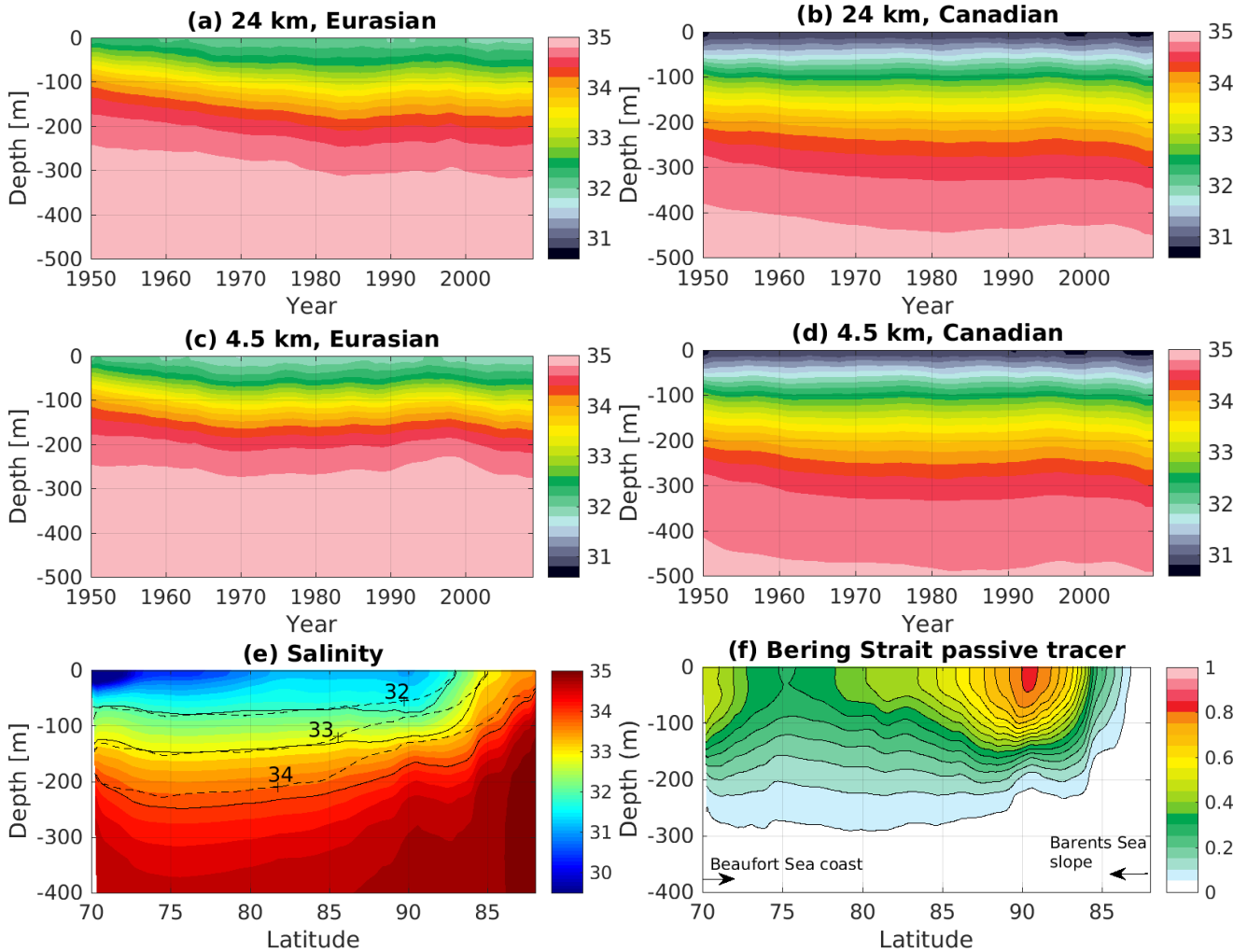
Figure 8. Hovmöller diagram of mean salinity for (a) the Eurasian Basin and (b) the Canadian Basin obtained in simulation LOW. (c),(d) are the same as (a),(b) but for simulation HIGH. (e) Salinity at the transect along the 140°W/40°E longitude averaged over the 1980-1999 period in simulation HIGH, shown by the color patch and solid contours. The dashed contours indicate the salinity at the beginning of the model simulation. (f) The same as (e) but for the passive tracer released in Bering Strait. The location of the transect is indicated in Fig. 1.
