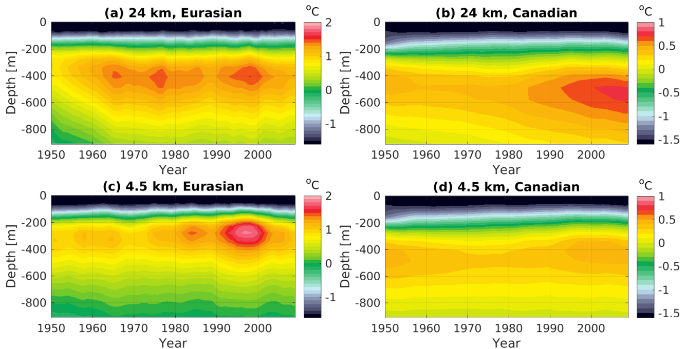
Figure 3. Hovmöller diagram of mean potential temperature for (a) Eurasian Basin and (b) Canadian Basin obtained in the simulation LOW. (c),(d) are the same as (a),(b) but for the simulation HIGH.
