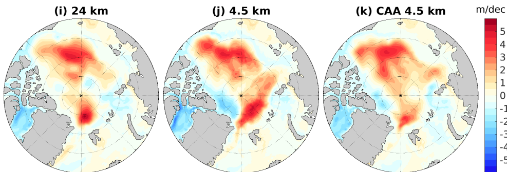
Figure 10. Mean liquid freshwater (FW) content (in m) for the period 1993–2002 for (a) LOW, (b) HIGH, (c) CAA HIGH, and (d) observation of Rabe et al. (2011). Difference in liquid FW content between the periods 2003–2007 and 1993–2002 for (e) LOW, (f) HIGH, (g) CAA HIGH, and (h) observation. Linear trend of FW content (m/decade) for the period 1996–2009 for (i) LOW, (j) HIGH and (k) CAA HIGH. The FW content is calculated using a reference salinity of 34.8. The sensitivity experiment CAA HIGH is introduced to isolate the impact of resolution in the Canadian Arctic Archipelago (CAA) from that in the Arctic interior. It has resolution similar to LOW outside CAA, but the same resolution as in HIGH inside CAA.
