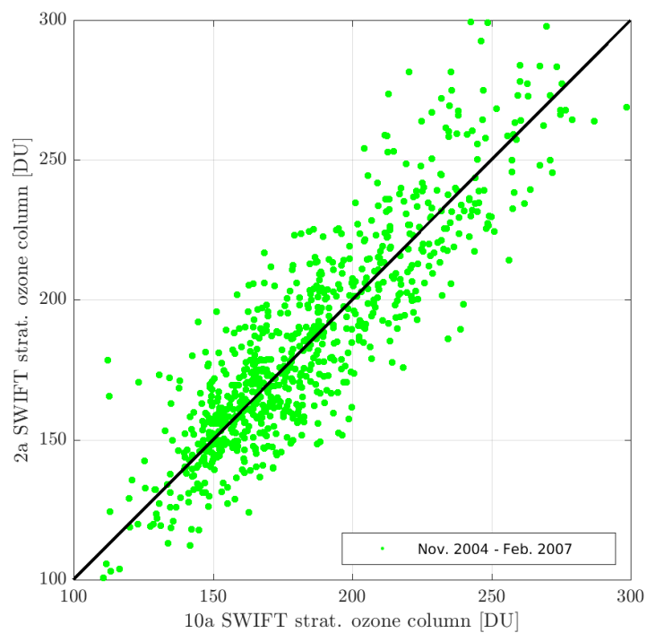
Fig. 2. Scatter plot showing daily averaged stratospheric ozone columns of the 10-year vs 2-year simulation.
