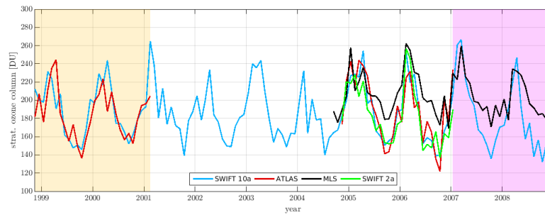
Fig. 1. Monthly mean values of the stratospheric ozone column (15 km – 32 km) over Potsdam, Germany. The bright green line shows the 2-year simulation.
