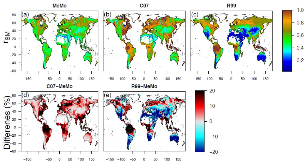
Figure 7. Soil moisture response ( r_{SM} ) of CH_4 oxidation simulated by models (a) MeMo, (b) C07 and (c) R99. Differences in model response expressed in percent are shown in panels (d) C07 minus MeMo, and (e) R99 minus MeMo.
