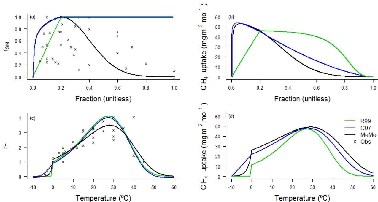
10 Figure 3: \text{CH}_4 uptake response factors (a, c) and uptake fluxes (b, d) as a function of soil moisture ( r_{SM} ) and temperature ( r_T ). Observations (shown as crosses) ( r_{SM} , Supplementary 1, Table S1; r_T , Supplementary 1, Table S2), MeMo (black line), C07 (blue line) and R99 (green line).
