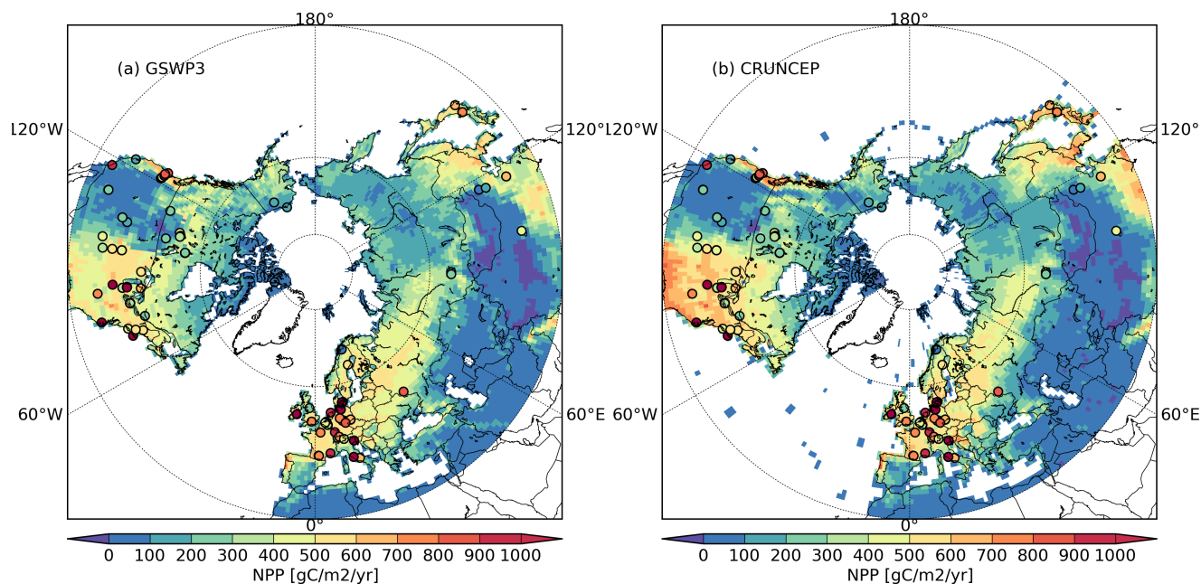
Figure 16. Mean annual NPP ( \text{gC m}^{-2} \text{yr}^{-1} ) simulated with (a) GSWP3 and (b) CRUNCEP forcings (background maps) compared to the site observations (color filled circles), on averaged over the period 2000-2007.
