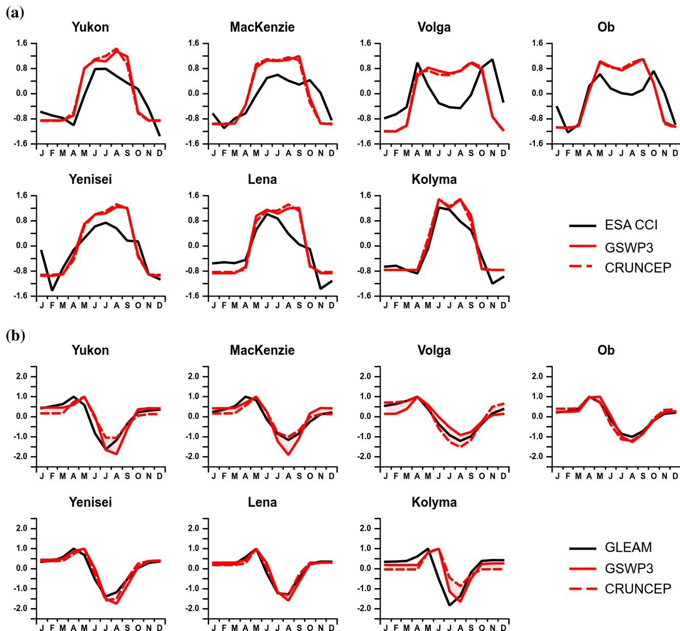
Figure 11. Monthly mean seasonal relative (a) topsoil (-) and (b) root soil moisture (-), both normalized by their multi-year standard deviation, simulated with the GSWP3 and CRUNCEP forcings over the seven basins (see Fig. 2b), averaged over the period 1981-2007. The results are compared with (a) satellite-derived observations from ESA CCI and (b) the GLEAM data driven model assimilated against satellite data.
