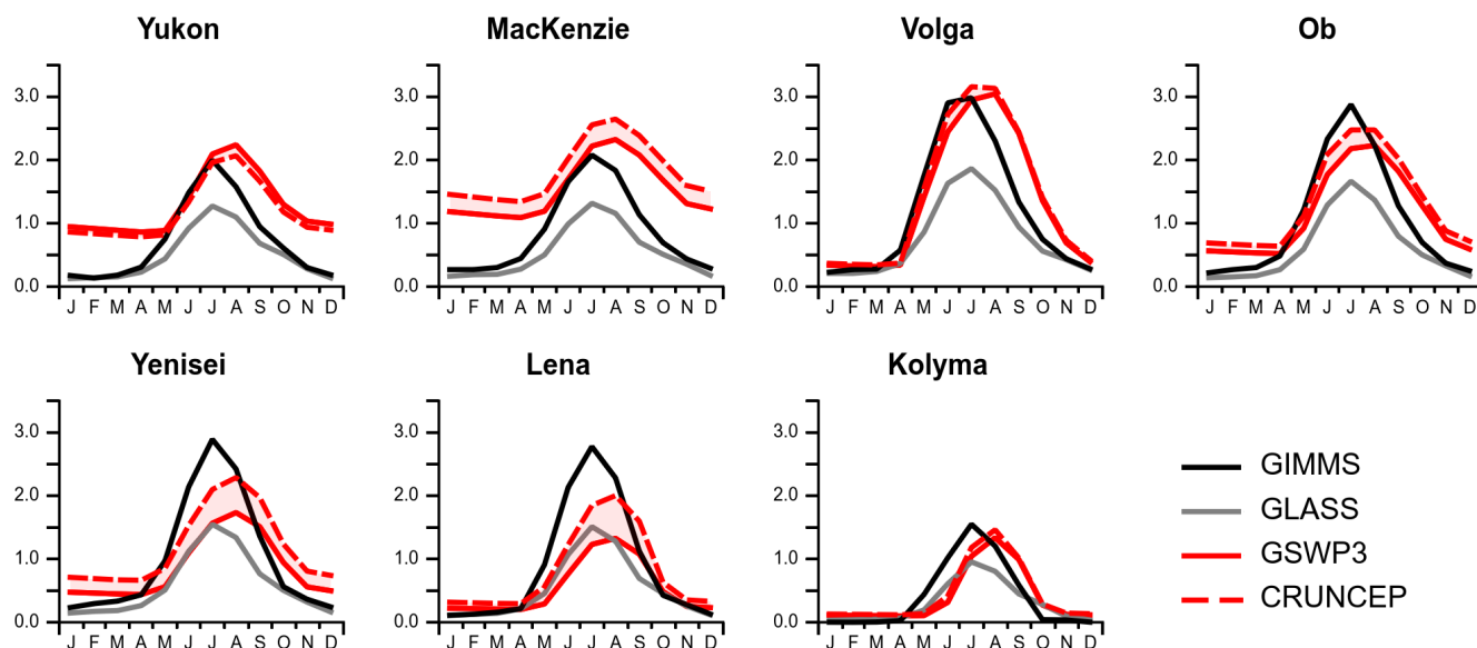
Figure 14. Monthly mean seasonal LAI (-) simulated with the two forcings compared to GIMMS and GLASS products over the seven basins (see Fig. 2b), averaged over the period 1981-2007.
