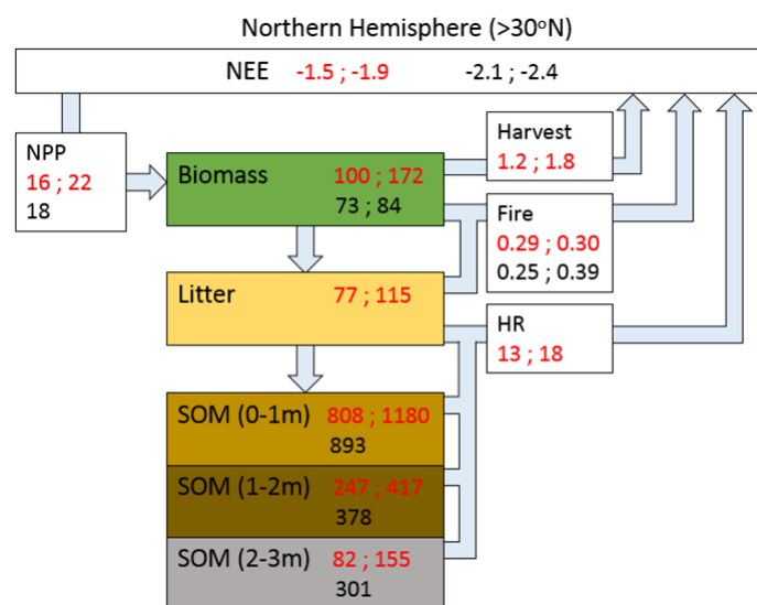
Figure 24. Annual mean land carbon fluxes ( \text{PgCyr}^{-1} ) and pool sizes ( \text{PgC} ), averaged over the terrestrial domain higher than 30^\circ\text{N} , for the period 2000-2007. The red numbers are the results of the model forced by (left) GSWP3 and (right) CRUNCEP. The black numbers are from observation-based estimates used in the text : NPP from MODIS (NTSG), fire emissions from (left) GFED4s and (right) GFAS datasets, harvest fluxes include crop harvest and wood product decay in the model (for simplicity the change in wood product pools is not represented), NEE from the two atmospheric inversions (left) Jena CarboScope and (right) CAMS, forest biomass from (left) Avitabile et al. (2016) and (right) Thurner et al. (2014), soil carbon from NCSCD (Hugelius et al., 2013) in permafrost regions and HWSD in non-permafrost regions.
