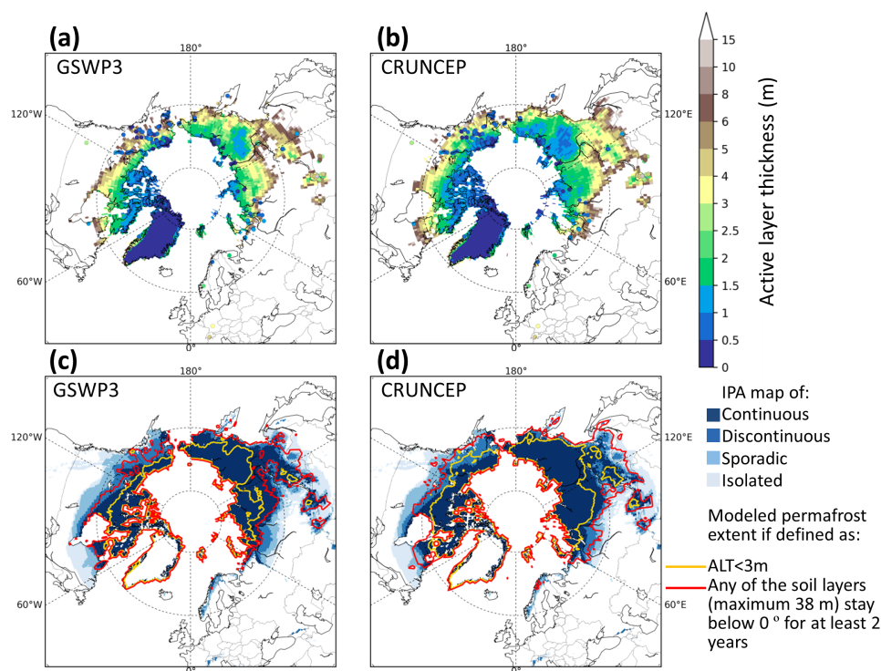
Figure 8. Active layer thickness (ALT in m) from the (a) GSWP3 and (b) CRUNCEP-forced simulation (background maps), compared to the observed ALT from the CALM network (color filled circles), averaged over the period 1990–2007. Permafrost extent from the (c) GSWP3 and (d) CRUNCEP-forced simulation according to two different definitions (yellow and red lines) on top of the IPA permafrost map (Brown et al., 2002).
