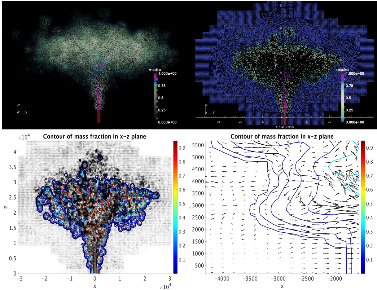
Figure 10. Mass fraction for t = 500s after eruption. Figures on the first row are visualization of SPH simulation results. The figure on the up right corner is visualization of a slice of the computational, whose thickness is around 10000m . The lowest portion of the plume represents erupted material in eruption vent (the underground portition). Figures at the second row show contour of mass fraction and velocity quiver on x - z plane. These figures are plotted utilizing post-processed data (see Appendix A). The contour level in the plot are 0.00001, 0.0001, 0.001, 0.1, 0.3, 0.75, 0.95 . The figure on the lower right corner is a zoomed view of velocity quiver showing plume expansion and entrainment of air.
