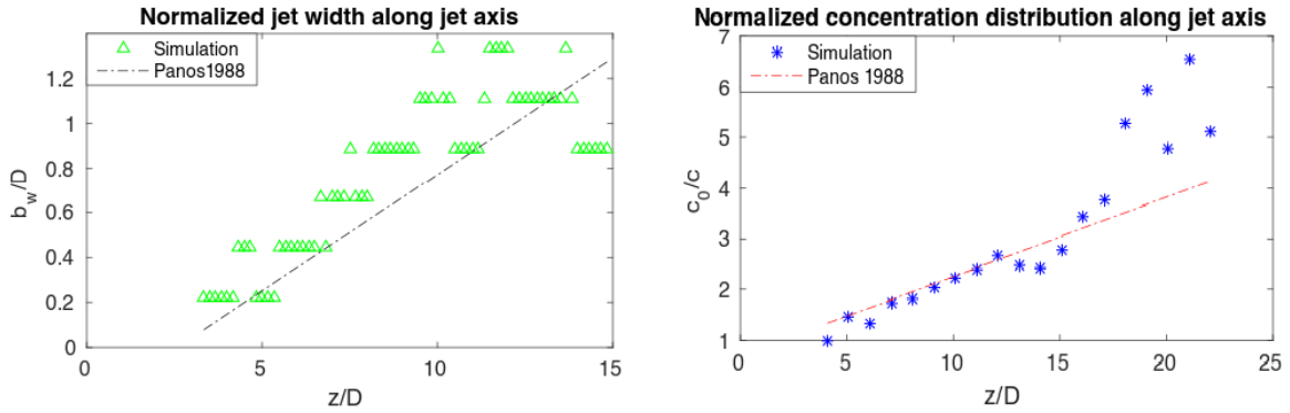
Figure 8. The left plot is normalized jet width (which determined based on velocity) along the centerline. The right plot shows normalized concentration along the centerline.
