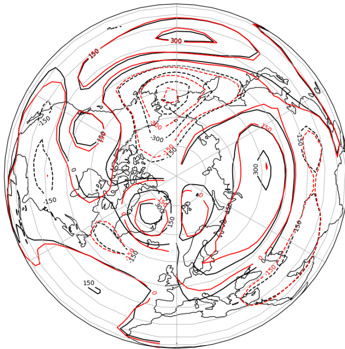
Figure A3: Northern Hemisphere annual mean 800 hPa geopotential height anomalies relative to the zonal average for the standard version of iLOVECLIM (CTRL – red) and the iLOVECLIM that includes a downscaling (DOWN, with z_q=2000\text{m} , \alpha_q^{\text{min}}=0.8 and f_s=0.6 – black).
