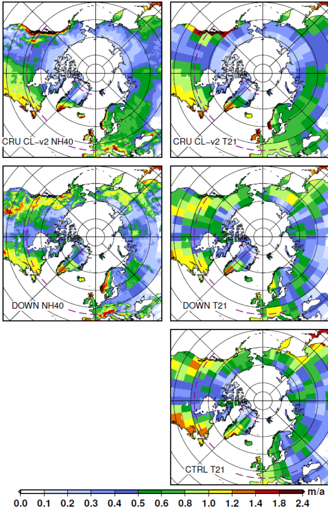
Figure A: Northern Hemisphere annual mean precipitation rate (m/yr) in: CRU CL-v2 (top), the iLOVECLIM that includes a downscaling (middle, with z_q=2000\text{m} , \alpha_q^{\text{min}}=0.9 and f_s=0.6 ) and the standard version of iLOVECLIM (bottom, CTRL). The left panel corresponds to data on the high resolution grid, whilst on the right data are aggregated to T21 resolution. The dashed purple lines stand for the selected transects used for discussion.
