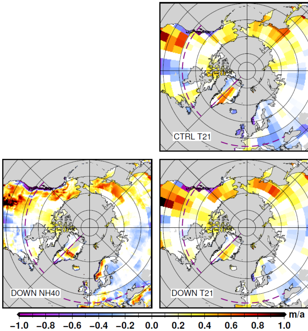
Figure A2: Northern Hemisphere annual mean precipitation rate difference (m/yr) from CRU CL-v2: standard version of iLOVECLIM (CTRL) and the iLOVECLIM that includes a downscaling (DOWN, with z_q=2000\text{m} , \alpha_q^{\text{min}}=0.8 and f_s=0.6 ). The left panel corresponds to data on the high resolution grid, whilst on the right the data are aggregated to T21 resolution.
