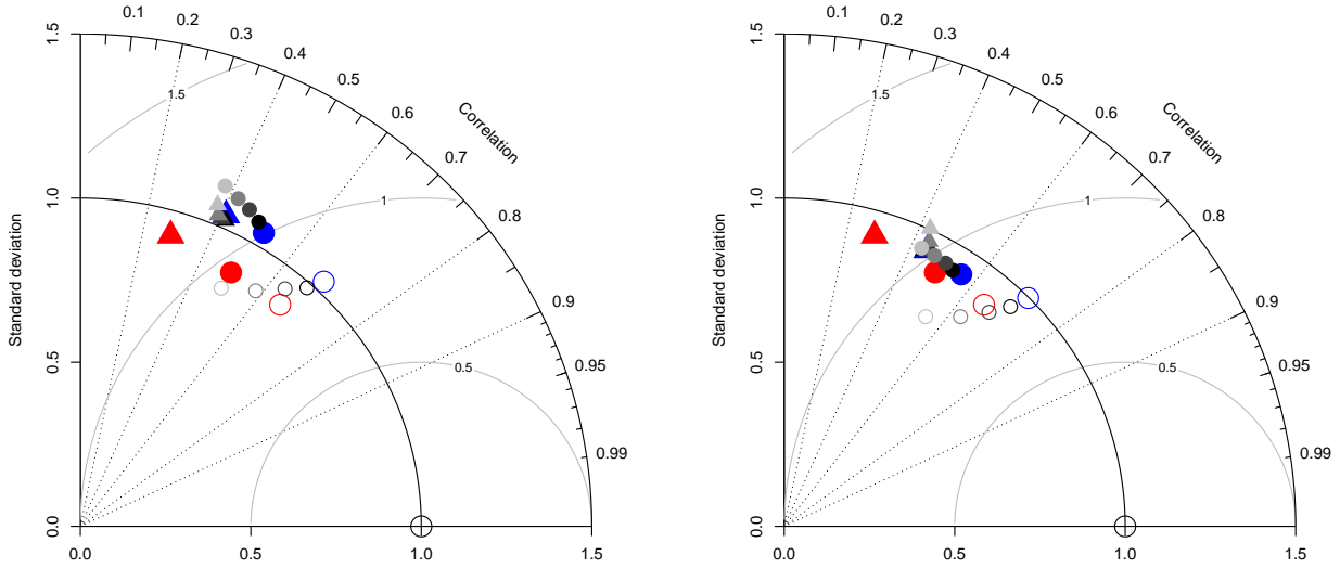
Figure 10. Normalised Taylor diagrams on the CRU CL-V2 annual mean precipitation rate for the standard CTRL experiment (red) and a series of DOWNS experiments (grey and blue). The circles depict the score when all grid points are considered, whilst the triangles stand for points with an elevation greater than 800 m. The filled symbols correspond to the Taylor Diagram computed on the high resolution grid whilst the symbols outlined-only are for the T21 grid. All the DOWNS experiments presented here use z_q = 2000m . The different shades of greys are for different \alpha_q^{min} ranging from 0.75 (dark) to 0.9 (light), for f_s = 1.0 (left) and f_s = 0.6 (right). DOWNS with z_q = 2000m , \alpha_q^{min} = 0.7 and f_s = 1.0 (left) and DOWNS with z_q = 2000m , \alpha_q^{min} = 0.7 and f_s = 0.6 (right) are in blue. In this figure, the metrics (standard deviation, correlation and root mean square error) are computed from the annual mean climatic variables. The standard deviation in the observations is used to normalise the standard deviations and the root mean square error.
