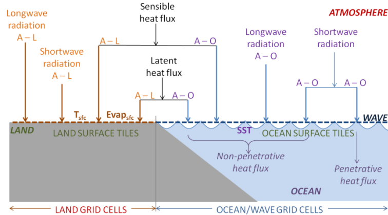
(c) UKC2 freshwater exchanges
