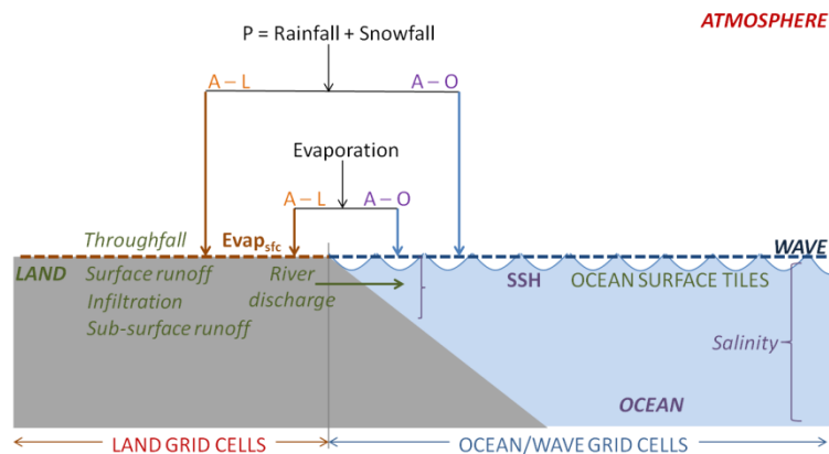
Figure 2: Summary of instantaneous fields exchanged each hour in the UKC2 coupled simulation categorised as (a) momentum, (b) heat and (c) freshwater exchanges between atmosphere-land (UM-JULES), ocean (NEMO) and wave (WAVEWATCH III) components.
