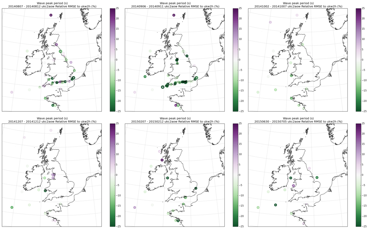
5 Figure 14: Differences in case study wave model RMSE statistics for wave peak period, comparing statistics computed for the fully coupled UKC2aow simulation as a % difference relative to the wave-only UKW2h runs with high resolution wind forcing. Green sites indicate an overall reduction in RMSE relative to the control. Results are shown for 5-day case study periods in (a) August 2014, (b) September 2014, (c) October 2014, (d) December 2014, (e) February 2015 and (f) July 2015. RMSE statistics are computed comparing UKC2aow and UKW2h model outputs with in-situ observations. Note that only an inner section of the domain is presented for clarity.
