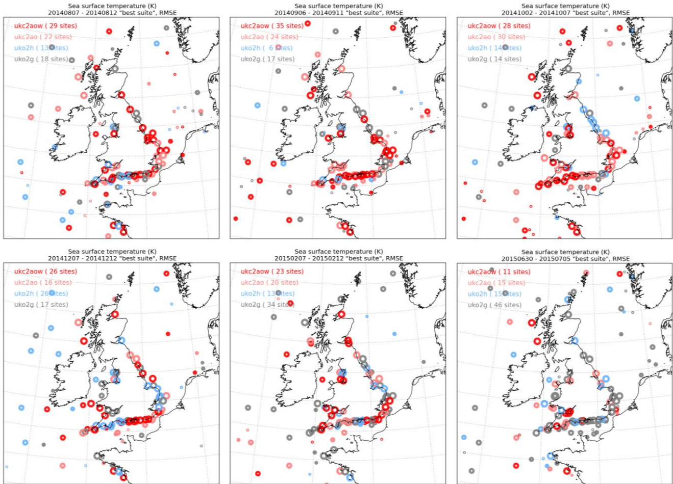
Figure 10: Distribution of in-situ observation sites for which each of UKC2aow, UKC2ao, UKO2h or UKO2g ocean model SST outputs provided the lowest RMSE statistic for each 5-day case study. Note that only an inner section of the domain is presented for clarity.
