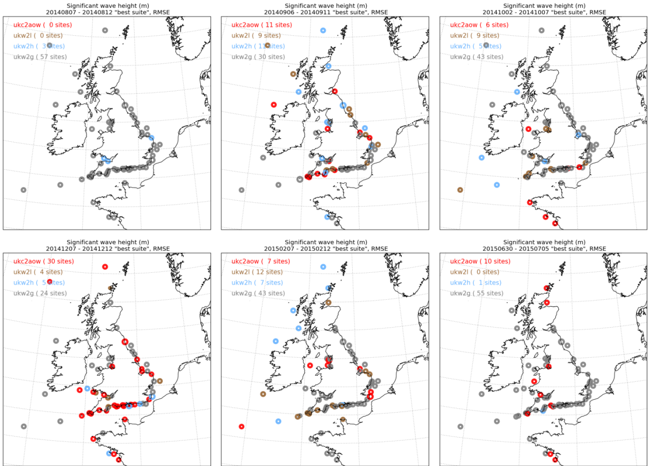
Figure 12: Distribution of in-situ observation sites for which each of UKC2aow, UKW2l, UKW2h or UKW2g wave model significant wave height outputs provided the lowest RMSE statistic for each 5-day case study. Note that only an inner section of the domain is presented for clarity.
