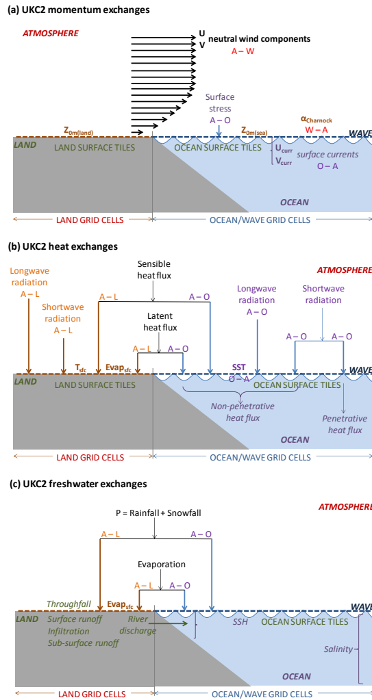
5 Figure 2: Summary of time-averaged fields exchanged each hour in the UKC2 coupled simulation categorised as (a) momentum, (b) heat and (c) freshwater exchanges between atmosphere-land (UM-JULES), ocean (NEMO) and wave (WAVEWATCH III) components. The relevant bulk and flux variables listed in Table 1 are shown as being exchanged between components, with flux variables shown with arrows.
