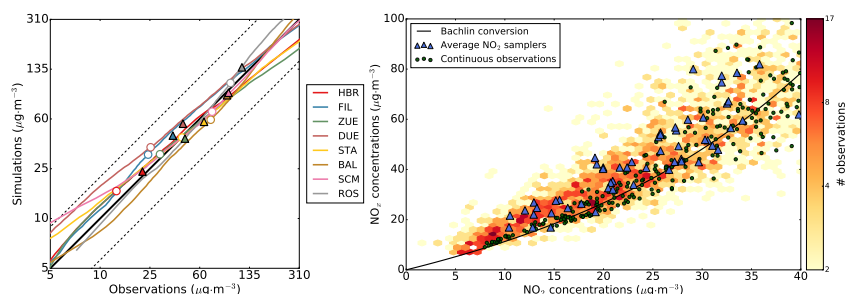
Figure 3. Comparison of observed and simulated \text{NO}_x and \text{NO}_2 concentrations. (left) Quantile-quantile plot of hourly \text{NO}_x concentrations at continuous sites. The solid and dashed black lines are the 1:1 line and the 1:2 and 2:1 lines, respectively. Filled triangles are the 2013–2014 mean and empty circles the median concentrations. Note the logarithmic scale of the plot. (right) Concentrations at passive samplers. Yellow to red coloured background show the comparison between 2-weekly observed \text{NO}_2 (x-axis) and corresponding simulated \text{NO}_x (y-axis). Triangles are the mean values per station averaged over the entire period 2013–2014. For comparison, green dots are the two-weekly averages of \text{NO}_2 and \text{NO}_x as observed at continuous sites. The black line is a “Bachlin”-type parametrization of the ratio between \text{NO}_x to \text{NO}_2 (Düring et al., 2011).
