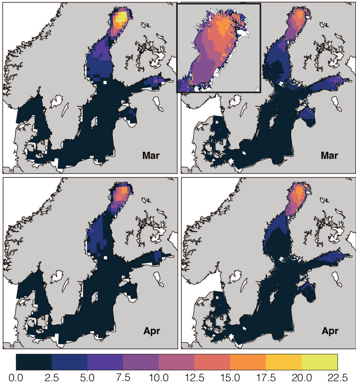
Figure 12. Climatological mean sea-ice ridge concentration in % for March and April, for the period 1961/62–1978/79. The left (right) column shows sea-ice ridge concentration for BASIS (NEMO-Nordic). For NEMO-Nordic the sea-ice ridge concentration is estimated from the fifth ice category. The inset shows a zoom over the Bothnian Bay for the simulated March distribution.
