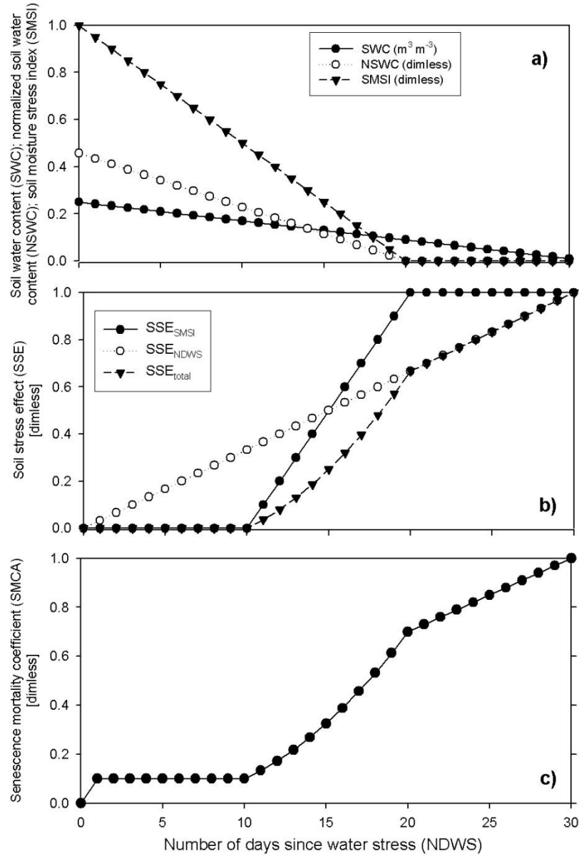
Figure 3. Demonstration of the senescence calculation with an example. a) Soil water content (SWC; black dots), normalized soil water content (NSWC; white dots) and soil moisture stress index (SMSI; black triangles) during 30 days of a hypothetical drought event. b) Soil stress effect based on soil moisture stress index ( \text{SSE}_{\text{SMSI}} ; black dots), soil stress effect based on number of days since water stress ( \text{SSE}_{\text{NDWS}} ) and total soil stress effect ( \text{SSE}_{\text{total}} ). c) Aboveground senescence mortality coefficient (SMCA).
