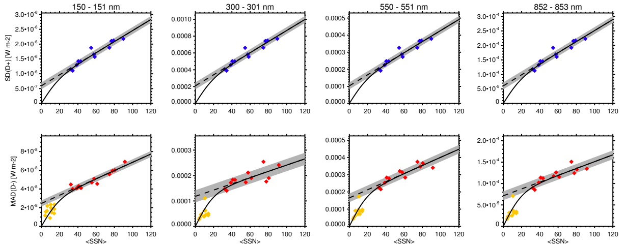
Figure 30. Regression of SD(D^+)_{SC} (top, blue symbols) and MAD(D^-)_{SC} (bottom, red symbols) to \langle SSN \rangle at wavelength bins centered at 150.5, 300.5, 550.5, and 852.5 nm (from left to right). The resulting linear fit is shown by dashed black lines, the grey shaded areas reflect the RMS errors. The solid black lines show the functional dependence used in the scaling after application of a non-linear correction for low \langle SSN \rangle values. MAD(D^-) values calculated from the low activity part of the solar cycles provide an estimate for very weak solar cycles and are shown with orange symbols (only lower panels).
