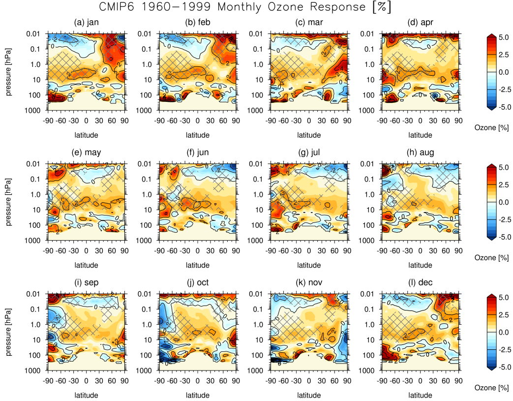
Figure 27. A preliminary estimate of the fractional (%) monthly solar-ozone response per 130 units of the F10.7cm flux in the CCMI Ozone Database for CMIP6 extracted using multiple linear regression for the period 1960-99 using the ozone mixing ratio files (vmro3_input4MIPs_ozone_CMIP_UReading-CCMI-1-0_gr_195001-199912.nc) downloaded from inputs4MIPs. The hatching denotes regions where the extracted solar-ozone response is estimated to be significantly different from zero at the 95% confidence level. Please note that the details of the CMIP6 Ozone Database are still being finalised at the time of writing and we refer readers to Hegglin (2016) for further details.
