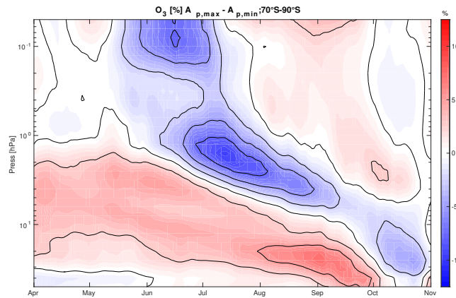
Figure 18. Ozone interannual variation due to geomagnetic forcing in 2005-2011 from EMAC model run using the MIPAS-derived UBC for \text{NO}_y . Shown are 27-day running means of the mean of the three years with highest – mean of the three years with lowest geomagnetic activity averaged over 70-90°S. EMAC results are in excellent agreement with \text{O}_3 observations using a three-satellite composite for the same period of time (see Figure 5 in Fytterer et al., 2015a).
