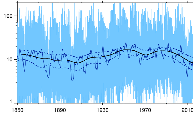
Figure 31. Decomposition of the reconstructed Ap index in the scaling procedure. Light blue: daily resolved Ap ; black: background component Ap^{bg} ; solid dark blue: annual component Ap^a ; dashed dark blue: scaling function SD(Ap^a) , multiplied by 1 and -1, used to scale the annual component.
