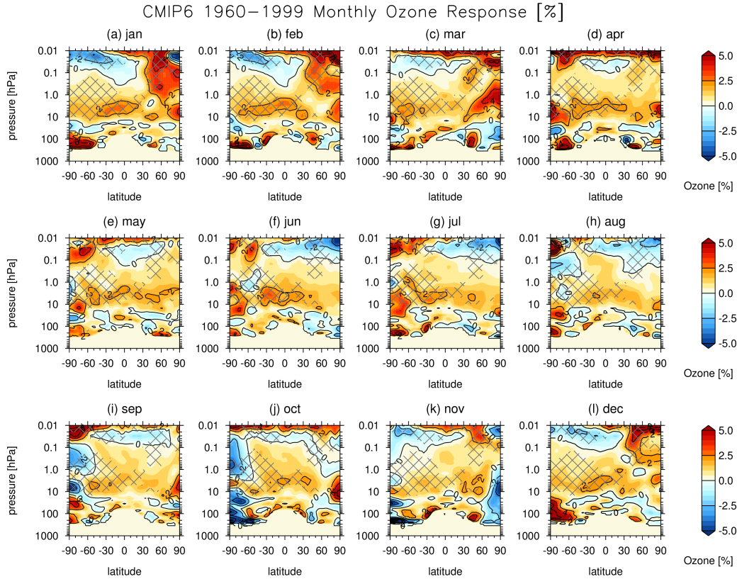
Figure 27. A preliminary estimate of the fractional (%) monthly solar-ozone response per 130 units of the F10.7cm flux in the CMIP6 Ozone Database-ozone database for the period 1960-99 using the ozone mixing ratio file (vmro3_input4MIPs_ozone_CMIP_UReading-CCMI-1-0_gr_195001-199912.nc) downloaded from inputs4MIPs. The hatching denotes regions where the solar-ozone response diagnosed using multiple regression analysis is found to be significantly different from zero at the 95% confidence level. Please note that the CMIP6 Ozone Database-ozone database for the future simulations has not been released at the time of writing and readers are referred to Hegglin et al. (2017) for further details.
