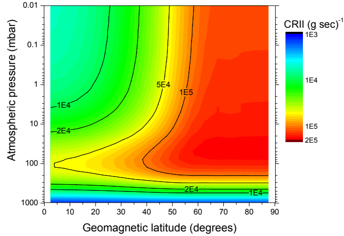
Figure 20. Calculated annual mean ion pair production rate for the year 2014 as a function of barometric pressure and geomagnetic latitude. Computations were done using the CRAC:CRII model.
