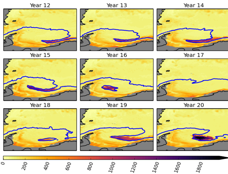
1 2 3 Figure 9: September mixed layer depth (m) and sea ice edge in GC2.1-N512O12 for years 12- 4 20 indicating the presence of a Weddell Sea polynya. The sea ice edge (marked in blue) is 5 based on a threshold of 15% ice concentration. 6 7
