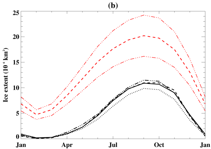
1 2 3 Figure 5: Seasonal cycle of sea ice extent in a) Northern and b) Southern hemisphere for years 4 11-20 compared against HadISST 1980-99 and with +/- 20% error bars denoted. 5
