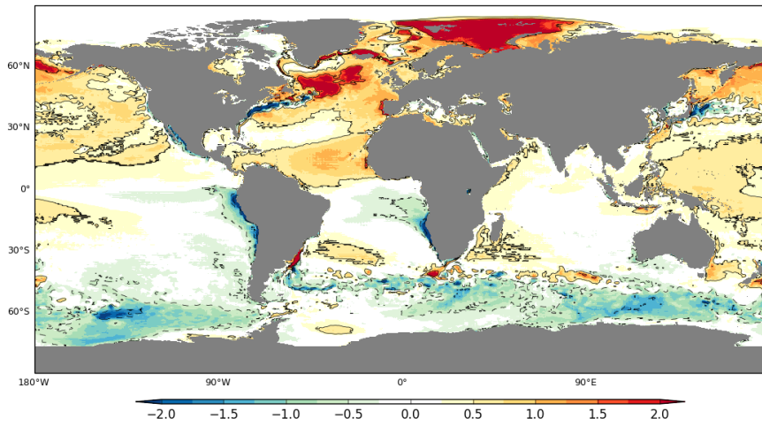
Figure 3: SST difference (°C) for years 11-20 between GC2.1-N512012 and GC2.1
