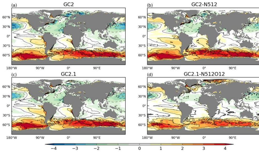
3 Figure 2: Differences between modelled SST from years 11-20 and observed SST from 4 HadISST ( ^{\circ}\text{C} ) for a) GC2, b) GC2-N512, c) GC2.1 and d) GC2.1-N512O12.
