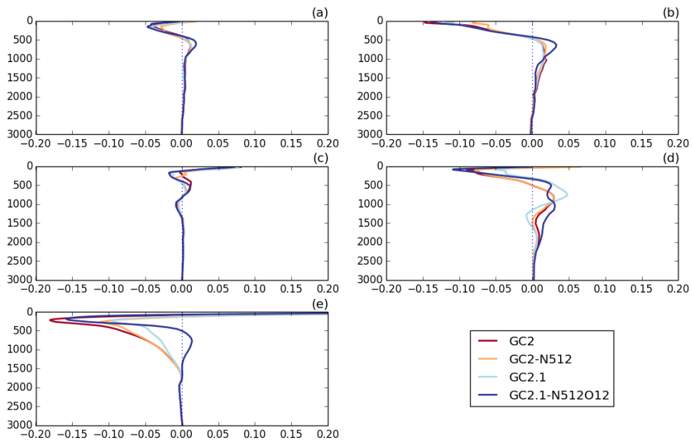
1 2 Figure 8: Area-weighted mean salinity difference (years 11-20 minus year 1; psu) for GC2, 3 GC2-N512, GC2.1 and GC2.1-N512O12 for a) global, b) 90S-30S, c) 30S-30N, d) 30N-90N, 4 e) 65N-90N. The vertical axis denotes depth (m).
