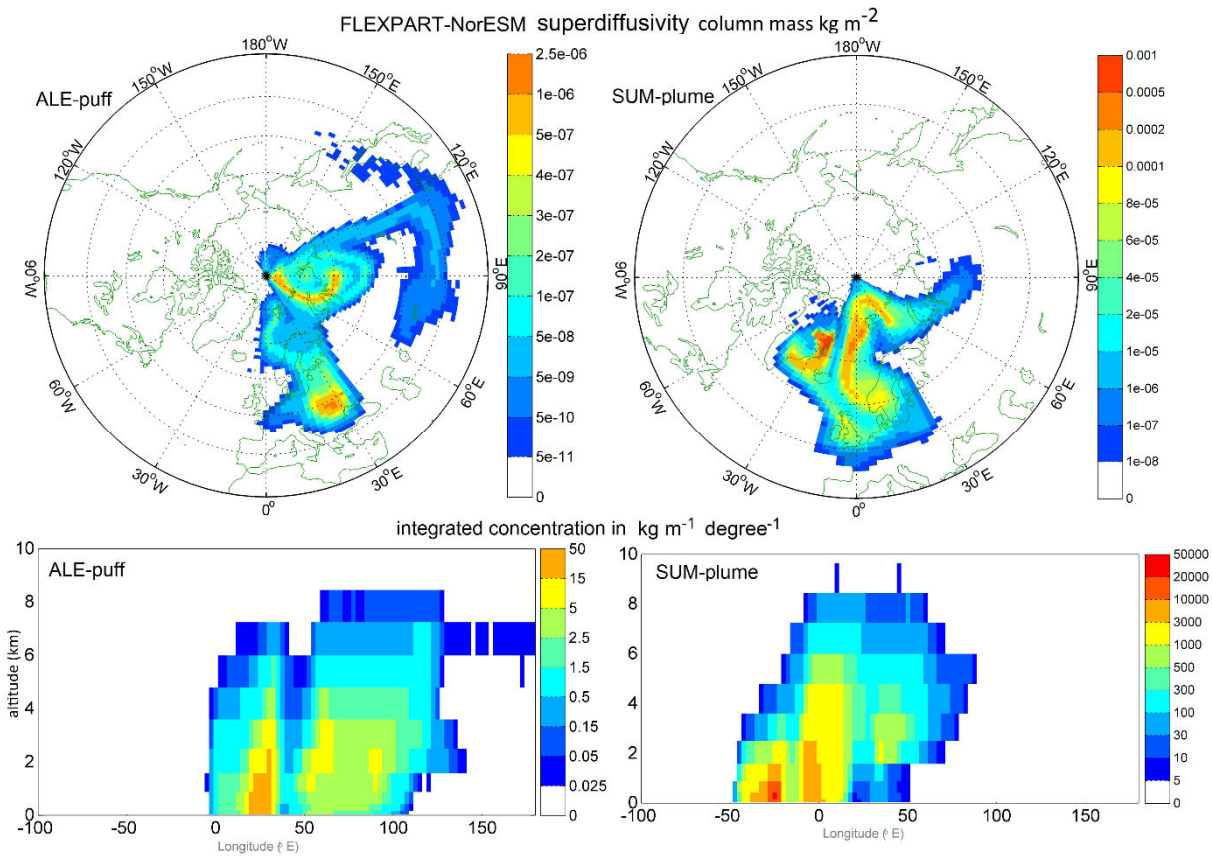
5 Figure 8. Results for the 30 minutes release from ALE (puff, left panels) and the continuous release from SUM (plume, right panels) as simulated with FLEXPART-NorESM/CAM with a tenfold increase in the horizontal diffusivity coefficients. Compare with NorESM results in Fig. 6 and 2.
