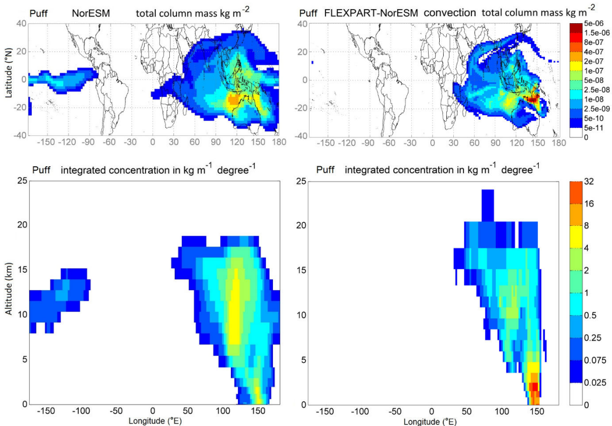
Figure 5. Puff dispersion after 144 hours from the GUI source. NorESM integrated solver results (left panels) and FLEXPART-NorESM/CAM results (right panels) are shown. The upper panels show maps of vertically integrated tracer concentrations, the lower panels show meridionally integrated tracer concentrations as a function of longitude and altitude.
