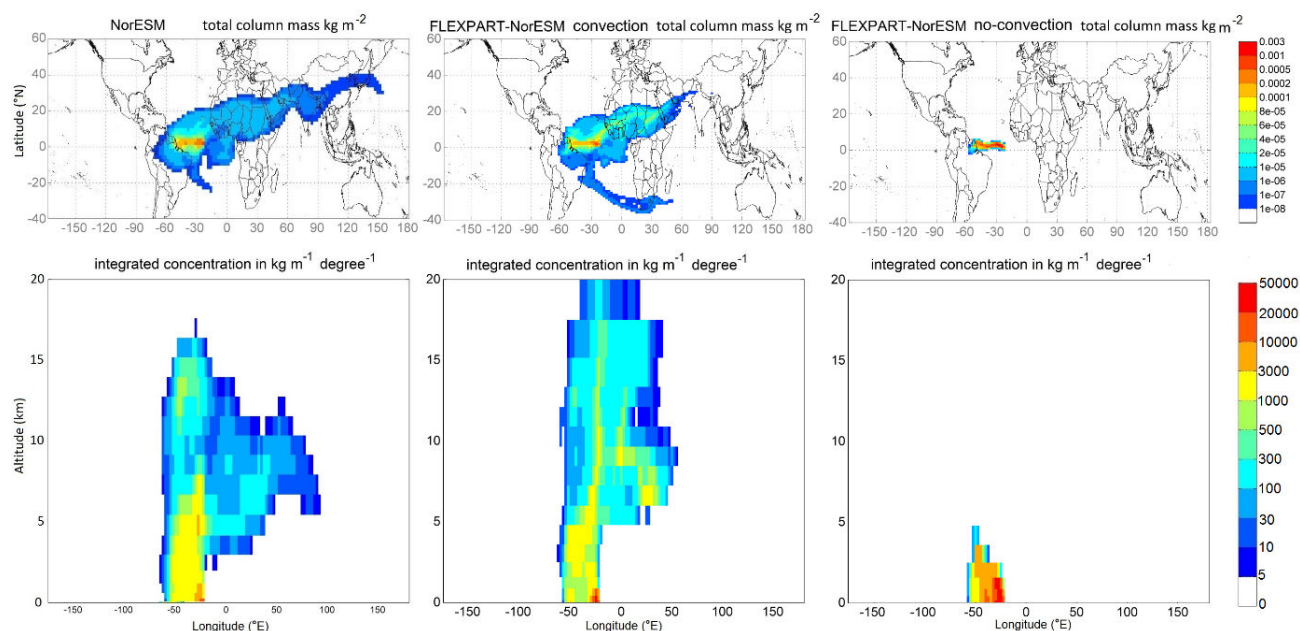
Figure 4. Continuous release from the EQA source. FLEXPART-NorESM/CAM results without convective scheme (right panels) and with convective scheme (central panels) versus NorESM integrated solver results (left panels) are shown. The upper panels show maps of vertically integrated tracer concentrations, the lower panels show meridionally integrated tracer concentrations as a function of longitude and altitude, 144 hours after the start of the simulation.
