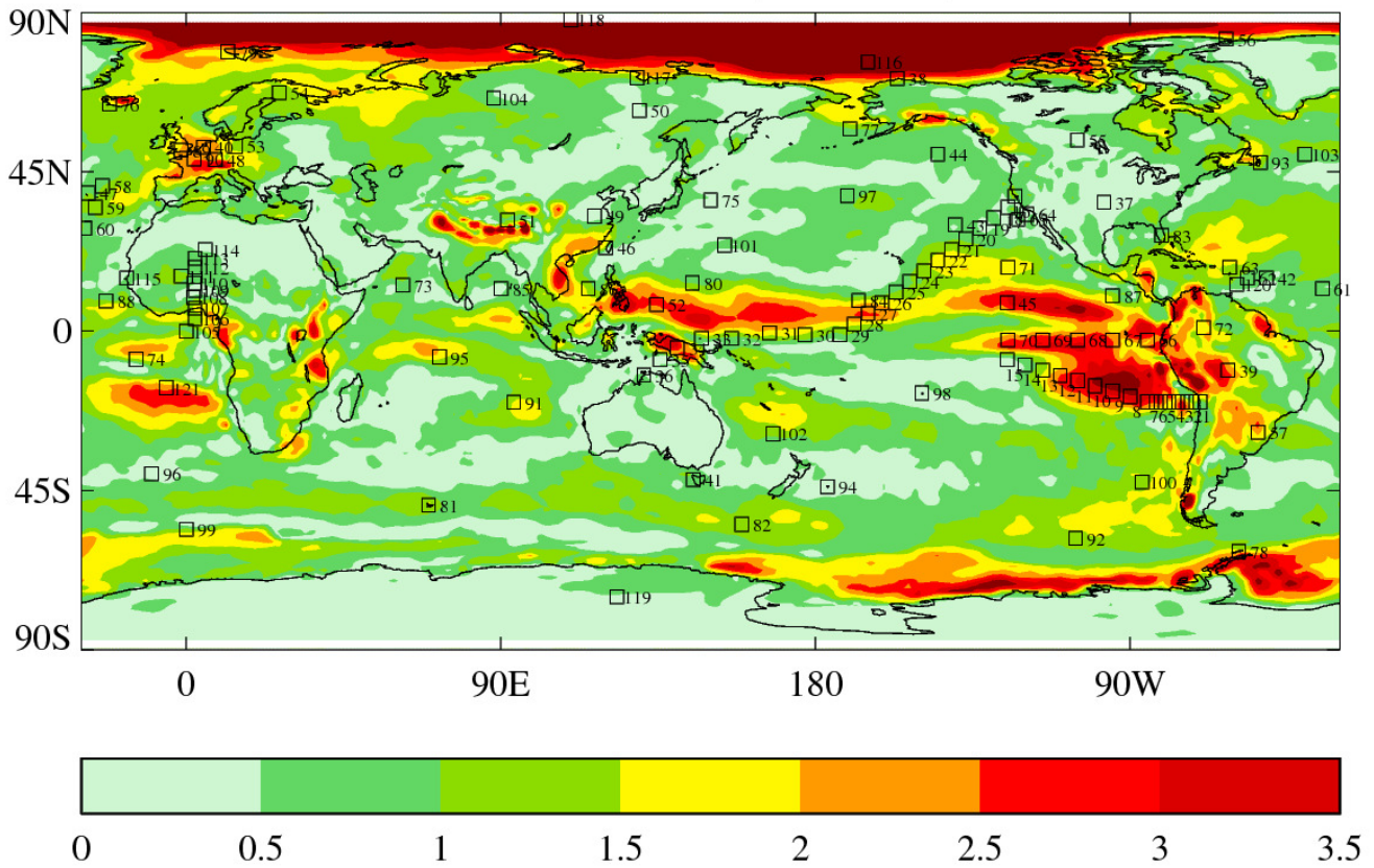
Figure 2. CFMIP-3/CMIP6 cfSites locations. The contours give an indication of inter-model spread in cloud feedback from the CFMIP-2/CMIP5 amip/amip4K experiments (please refer to Webb et al., 2015a for details).
