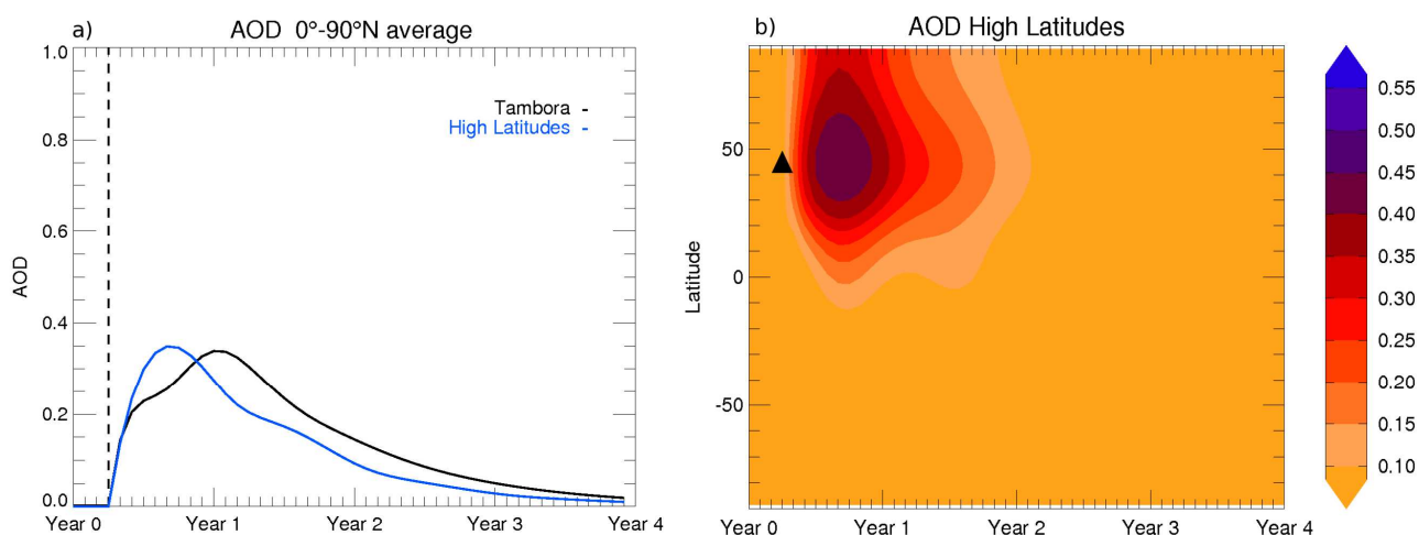
Figure 4: Consensus forcing for the volc-long-hlN experiment. (a) Northern Hemisphere-average aerosol optical depth (AOD) at 550 nm produced by the Easy Volcanic Aerosol module (EVA) for a 56.2 Tg equatorial eruption ( volc-long-eq , black line) and for a 28.1 Tg SO 2 Northern Hemisphere extra-tropical eruption ( volc-long-hlN , blue line). (b) Time-latitude plots of the AOD at 550 nm from EVA for the 28.1 Tg SO 2 Northern Hemisphere extra-tropical eruption. The black triangle shows latitudinal position and timing of the eruption.
