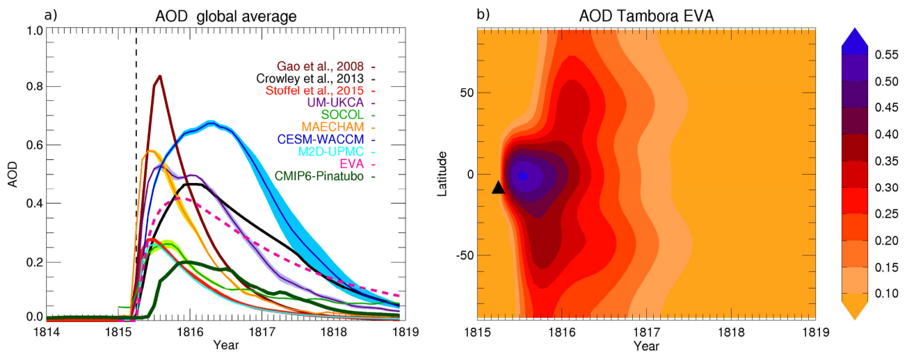
950 Figure 3: (a) Uncertainty in estimates of radiative forcing parameters for the 1815 eruption of Mt Tambora: global-average aerosol optical depth (AOD) in the visible band from an ensemble of simulations with chemistry climate models forced with a 60 Tg SO 2 equatorial eruption, from the Easy Volcanic Aerosol module (EVA) with 56.2 Tg SO 2 equatorial eruptions (magenta thick dashed line), from Stoffel et al. (2015), from Crowley and Unterman (2013), and from Gao et al. (2008, aligned so that the eruption 955 starts on April 1815). The estimate for the Pinatubo eruption as used in the CMIP6 historical experiment is also reported for comparison. (b) Time-latitude plot of the AOD in the visible band produced by EVA for a 56.2 Tg SO 2 equatorial eruption, illustrating the consensus forcing for the volc-long-eq experiment. The black triangle shows latitudinal position and timing of the eruption. Chemistry climate models are CESM (WACCM) (Mills et al., 2016), MAECHAM5-HAM (Niemeier et al., 960 2009), SOCOL (Sheng et al., 2015), UM-UKCA (Dhomse et al., 2014), CAMB-UPMC-M2D (Bekki, 1995; Bekki et al., 1996). For models producing an ensemble of simulations, the line and shading are the ensemble mean and ensemble standard deviation, respectively.
