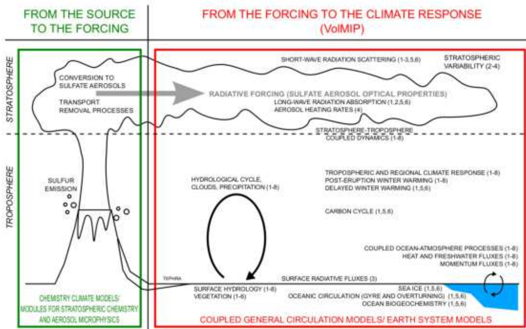
Figure 2: Illustrating the dominant processes linking volcanic eruptions and climate response, with an overview of VolMIP experiments: 1: volc-long-eq, 2: volc-pinatubo-full, 3: volc-pinatubo-surf, 4: volc-pinatubo-strat, 5: volc-long-hlN/-hlS, 6: volc-cluster-ctrl/-mill/-21C, 7: volc-pinatubo-slab, 8: volc-pinatubo-940 ini. The red box encompasses the processes related to the climatic response to volcanic forcing that are accounted for in VolMIP; the green box encompasses the processes regarding volcanic forcing that are neglected by VolMIP.
