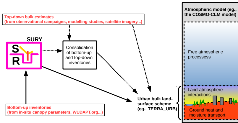
Figure 6. Outline Application outline of the Semi-empirical URban canoPY parametrization SURY implemented in an atmospheric model system . The main application flow of SURY is indicated with full arrows, whereas optional application flows are indicated with dashed arrows.
