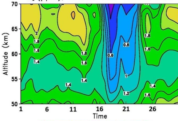
O 3 (ppm), WACCM-rSIC - 2005 Jan.
