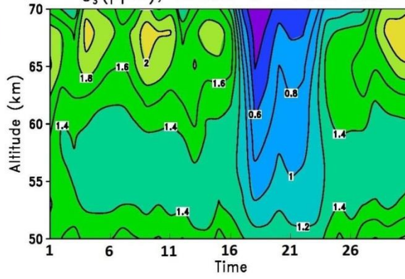
O 3 (ppm), WACCM - 2005 Jan.
