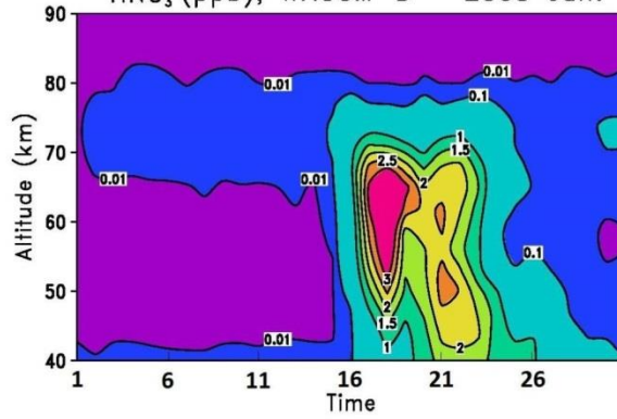
HNO 3 (ppb), WACCM - 2005 Jan.
