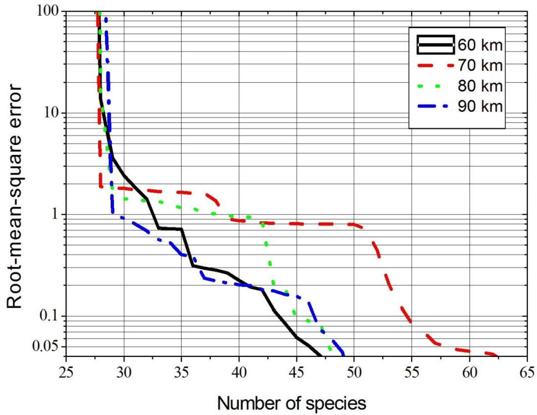
Figure 1. Root-mean-square (rms) error of all species as a function of number of species in the reduced mechanism 5 for the four selected altitudes (60, 70, 80 and 90 km).
