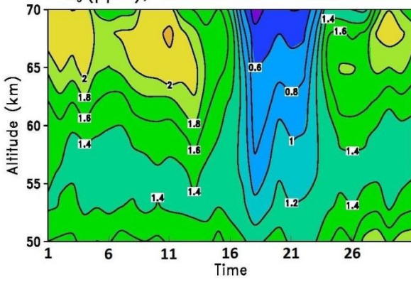
O 3 (ppm), WACCM-rSIC - 2005 Jan.
