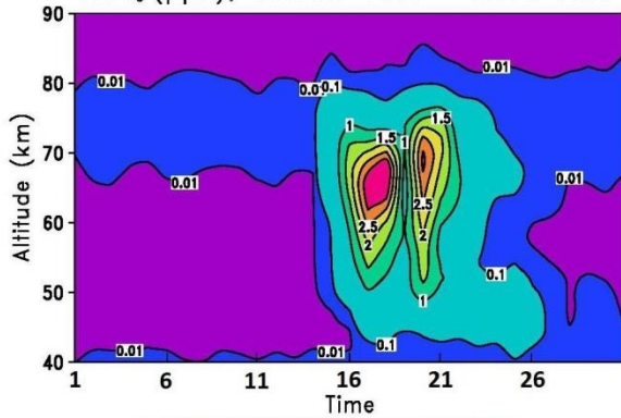
HNO 3 (ppb), WACCM-rSIC - 2005 Jan.
