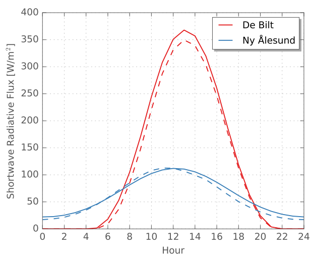
Figure 11. Long-term averages of diurnal courses of observed (dashed) and disaggregated (solid) shortwave radiation. Disaggregation is based on daily recordings of sunshine duration.
