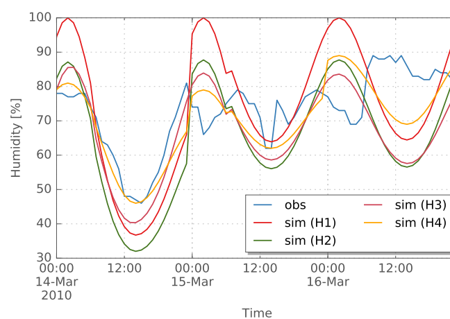
Figure 4. Example application of different humidity disaggregation models for Obergurgl. Observed and disaggregated time series are shown for relative humidity.
