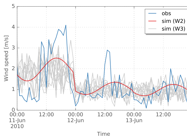
Figure 5. Example application of the wind disaggregation models W2 and W3 for Obergurgl. Observed and disaggregated time series are shown for wind speed. For option W3, 10 realisations are shown.
