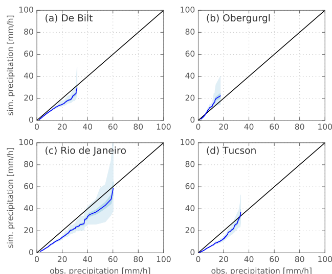
Figure 12. Modelled (blue) vs. observed (black) precipitation intensities for the 1% highest intensities derived using a split-sample test for the cascade model. For all panels the shaded areas refer to the standard deviation (dark blue) and range of values (light blue) computed for 100 realisations, respectively.
