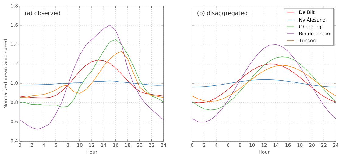
Figure 10. Long-term averages of diurnal courses of (a) observed and (b) disaggregated ‘normative’ wind speed. The ‘normative’ wind speed indicates the ratio of the long-term mean of the wind speed observed or modelled at a specified hour to the respective value averaged for the entire day. The period of time involved in this analysis is listed in Tab. 1 for each station.
