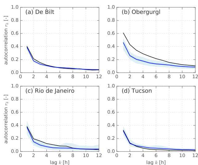
Figure 13. Autocorrelation r_k as function of time lag k (in hours) plotted for modelled (blue) and observed (black) precipitation time series. For all panels the shaded areas refer to the standard deviation (dark blue) and range of values (light blue) computed for 100 realisations, respectively.
