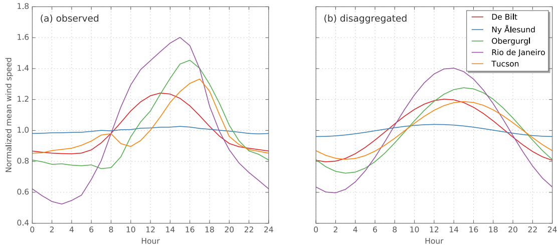
Figure 11. Long-term averages of diurnal courses of (a) observed and (b) disaggregated ‘normative’ wind speed ( W2 model ). The ‘normative’ wind speed indicates the ratio of the long-term mean of the wind speed observed or modelled at a specified hour to the respective value averaged for the entire day. The period of time involved in this analysis is listed in Tab. 1 for each station.
