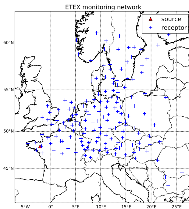
Figure 4. Domain of the ETEX experiment with source (red triangle) and receptors (blue crosses).
