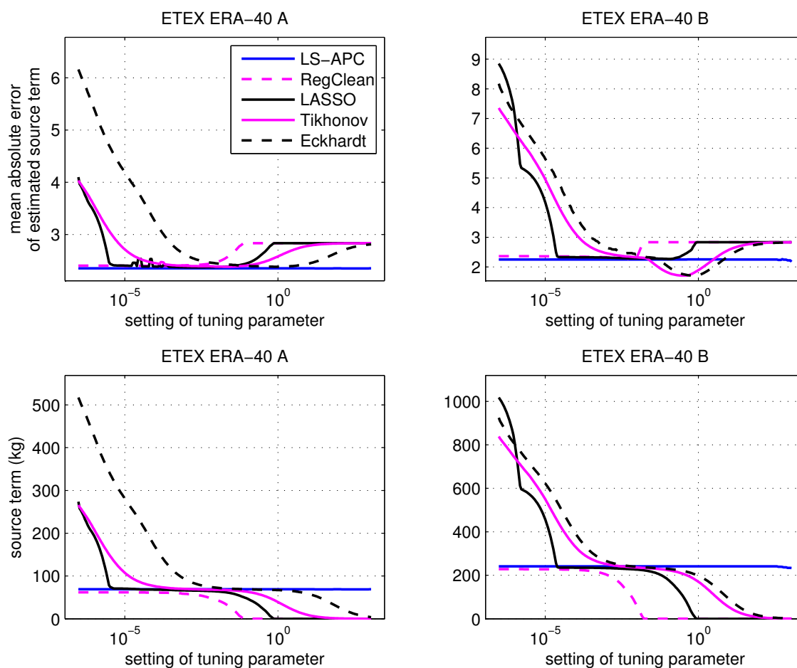
Figure 5. Comparison of sensitivity of the tested algorithms to the setting of the selected tuning parameter measured in terms of the mean absolute error metric (top row) and total estimated mass of the source term (bottom row) on data ETEX ERA-40 A and B.
