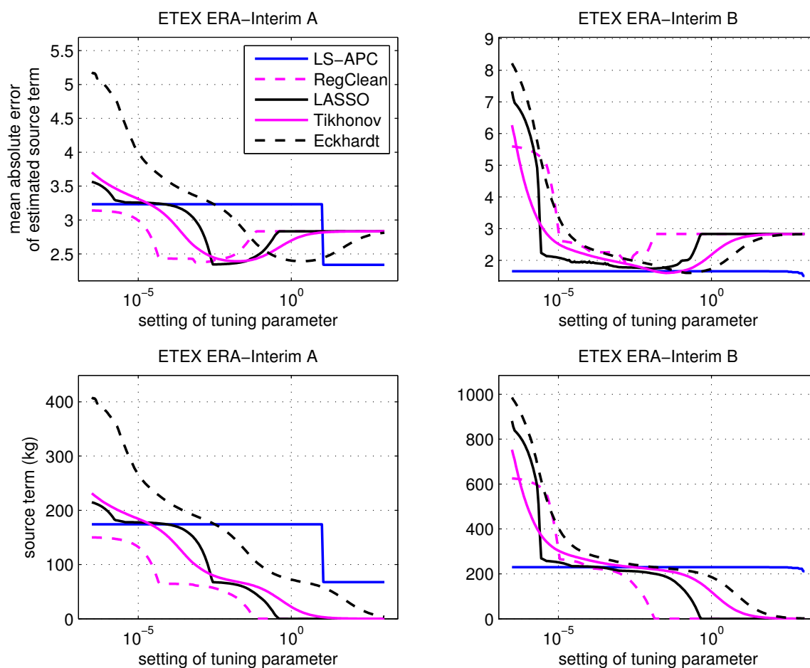
Figure 6. Comparison of sensitivity of the tested algorithms to the setting of the selected tuning parameter measured in terms of the mean absolute error metric (top row) and total estimated mass of the source term (bottom row) on data ETEX ERA-Interim A and B.
