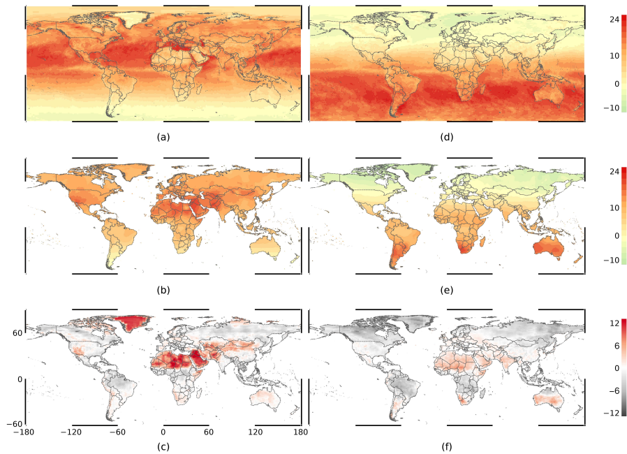
Figure 6. Global mean net downward surface radiation flux, \text{MJ m}^{-2} , for June (left) and December (right) 2000 CE from CERES EBAF (top) and the SPLASH model results (middle), and the differences between SPLASH and CERES EBAF (bottom). (a) CERES EBAF June 2000; (b) SPLASH June 2000; (c) difference between SPLASH and CERES EBAF June 2000; (d) CERES EBAF December 2000; (e) SPLASH December 2000; and (f) difference between SPLASH and CERES EBAF December 2000. Color bars on the right are linear interpolations of results in \text{MJ m}^{-2} . Differences in red indicate higher SPLASH model results.
