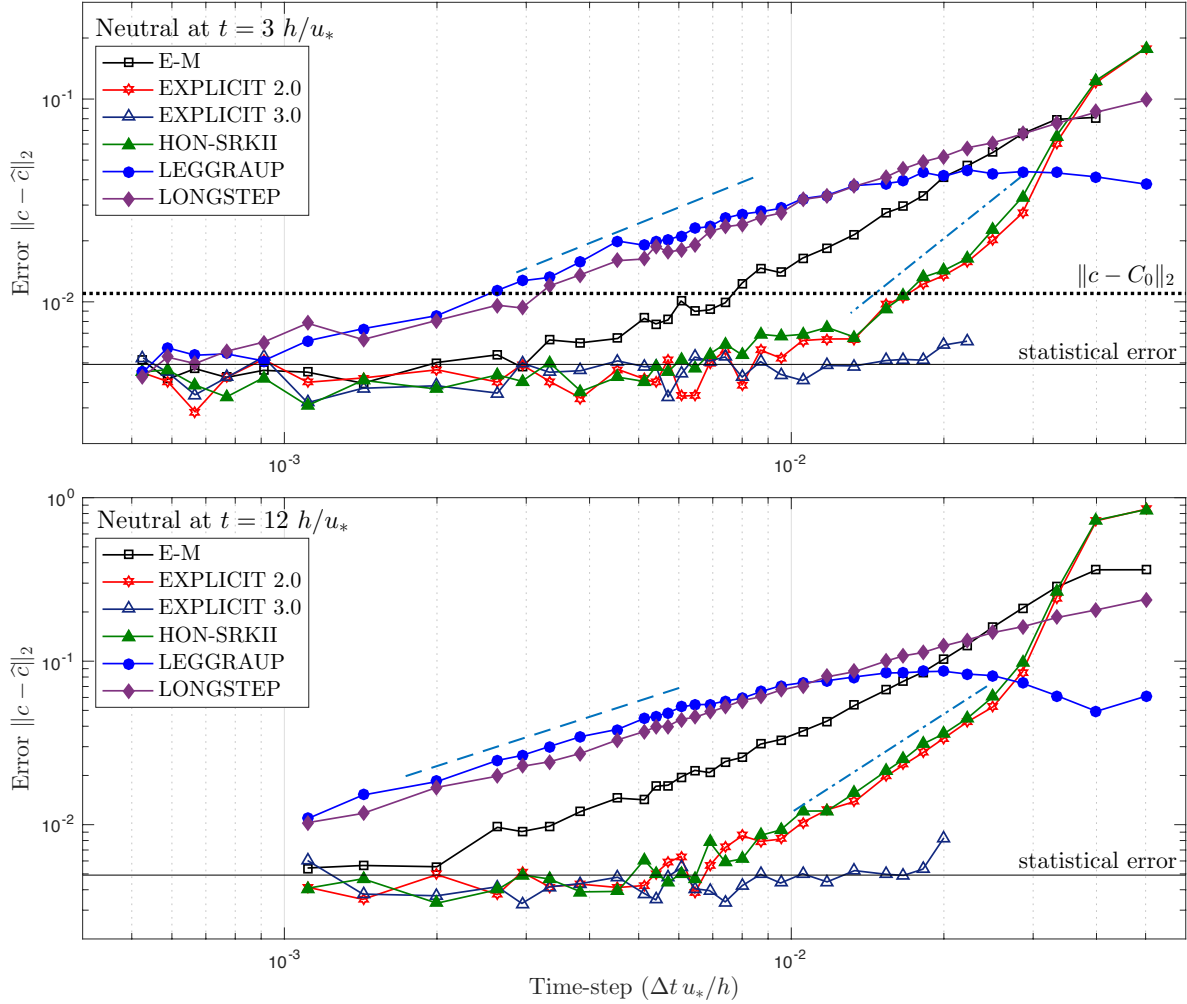
Figure 6. L_2 -error (20) as a function of non-dimensional time-step \Delta t u_* / h for the neutral ABL test case integrated at intermediate time t = 3 h/u_* (upper panel) and at late time t = 12 h/u_* (lower panel). From left to right, blue lines of slopes 1, 2 and 3 are plotted for reference.
