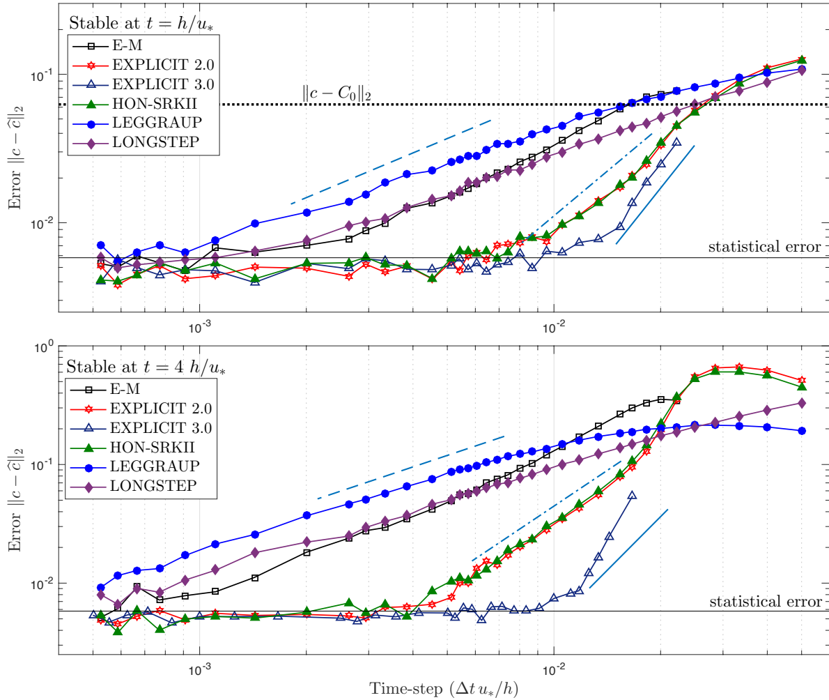
Figure 5. L_2 -error (20) as a function of non-dimensional time-step \Delta t u_*/h for the stable ABL test case integrated at intermediate time t = 1h/u_* (upper panel) and at late time t = 4h/u_* (lower panel). From left to right, blue lines of slopes 1, 2 and 3 are plotted for reference.
