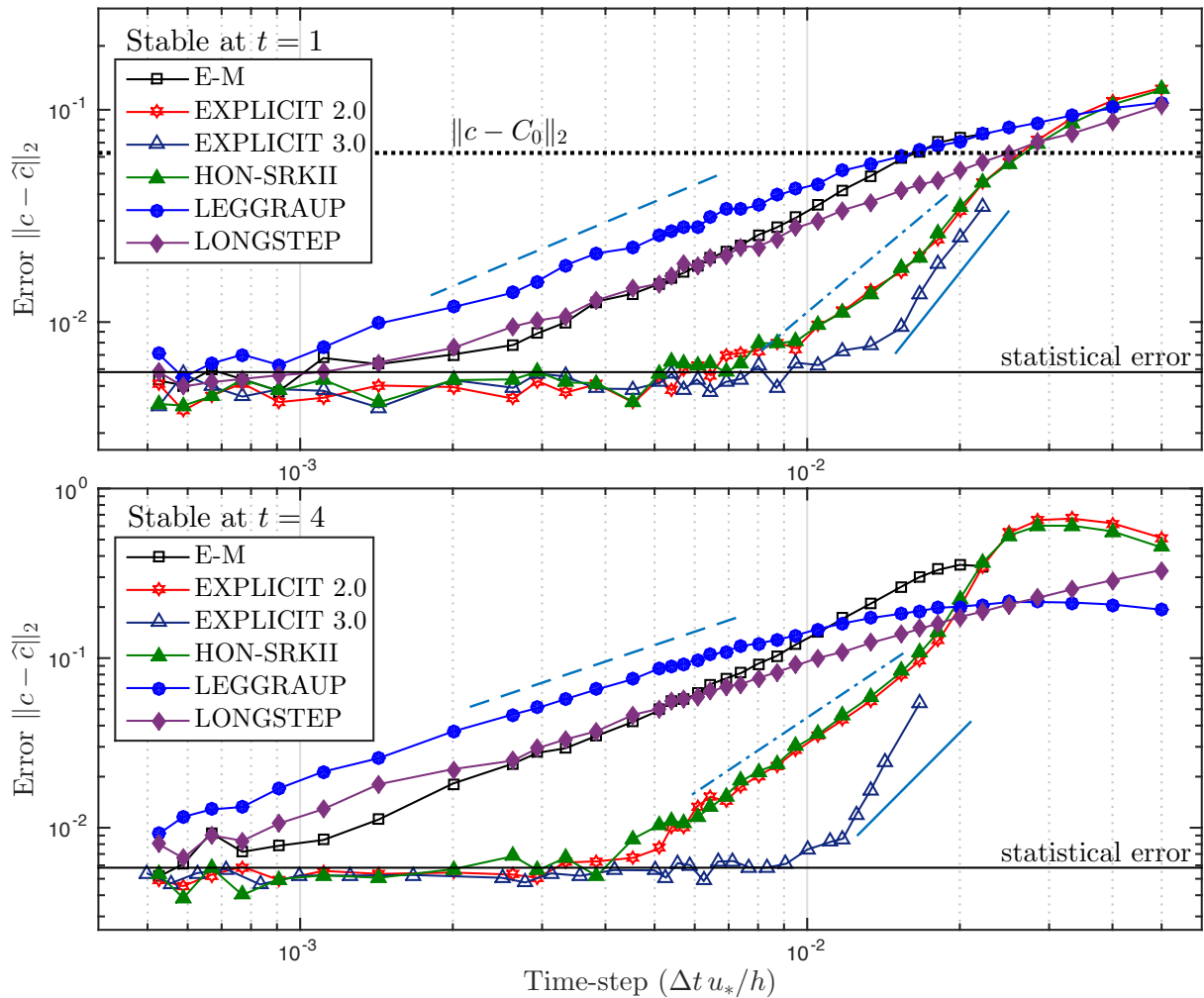
Figure 5. L_2 -error (20) as a function of non-dimensional time-step \Delta t u_*/h for the stable ABL test case integrated at intermediate time t = 1h/u_* ( t = h/u_* ) (upper panel) and at late time t = 4h/u_* (lower panel). From left to right, blue lines of slopes 1, 2 and 3 are plotted for reference.
