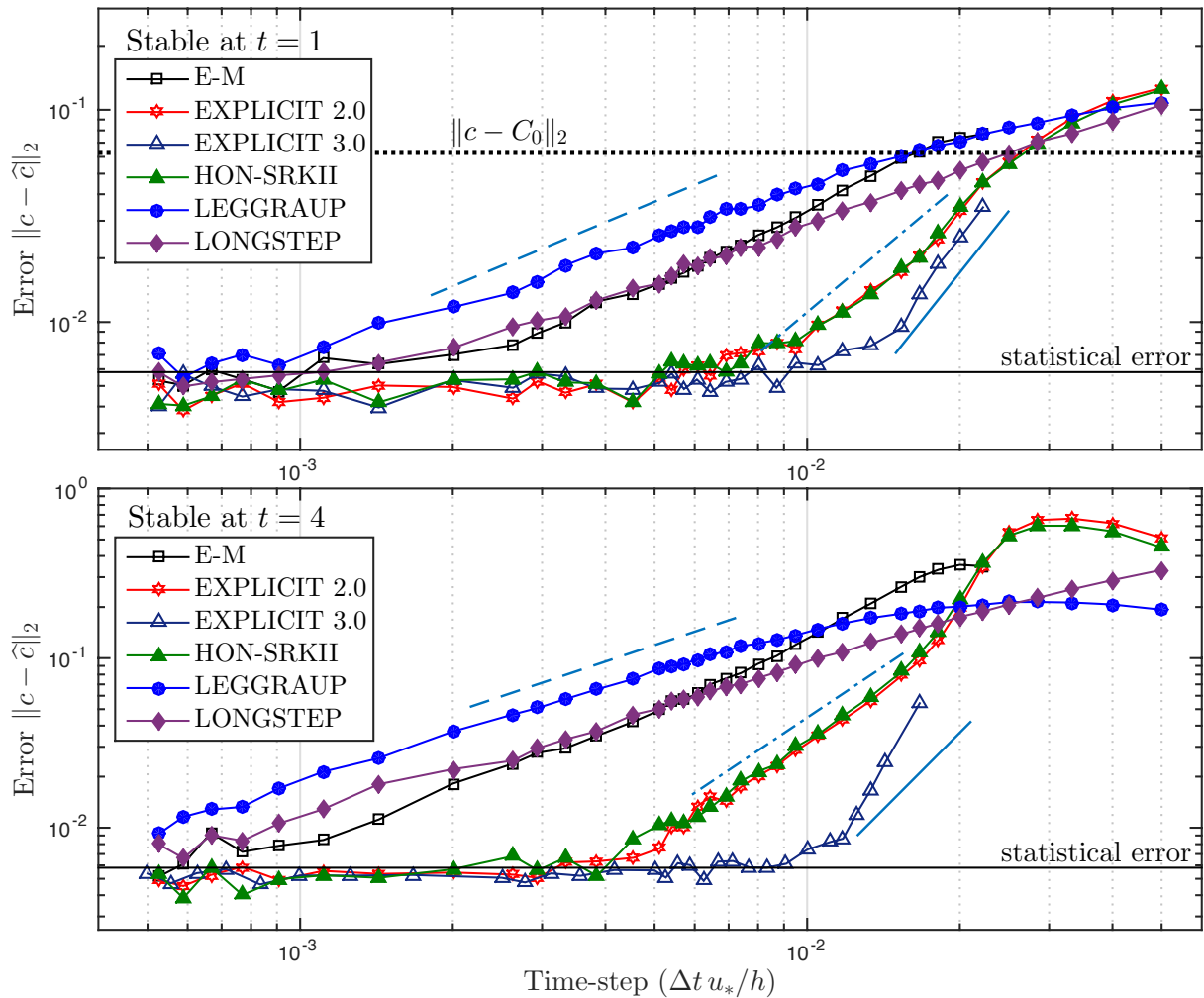
Figure 5. L_2 -error (20) as a function of non-dimensional time-step \Delta t u_* / h for the stable ABL test case integrated at intermediate time t = 1h/u_* ( t = h/u_* ) (upper panel) and at late time t = 4h/u_* (lower panel). From left to right, blue lines of slopes 1, 2 and 3 are plotted for reference.
