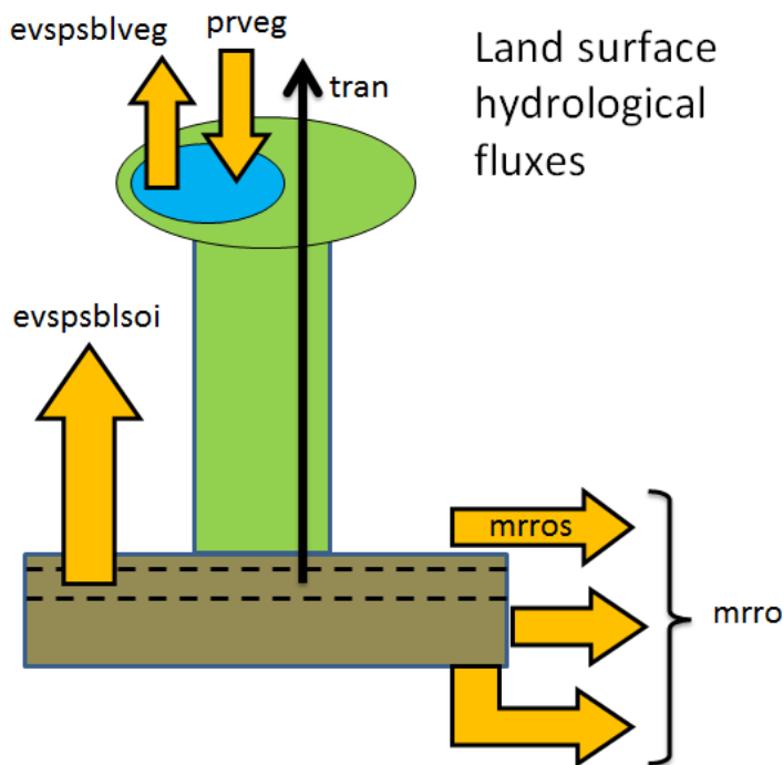
Figure 10: Requested land surface hydrological flux variables.
