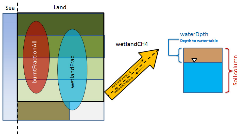
Figure 12: Fire and wetland variables. Other than burntFractionAll, all other variables are requested as Tier 2 variables.
