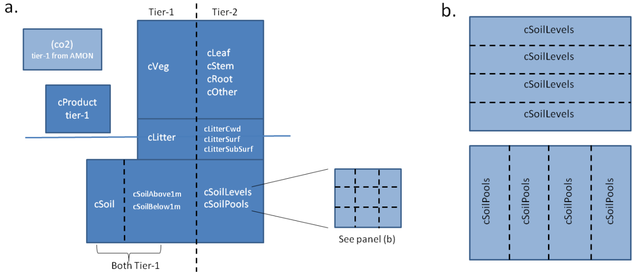
Figure 5: (a) Requested tier-1 and tier-2 variables representing land carbon pools. Although not a land carbon quantity, atmospheric CO 2 is shown here for completeness. (b) Detailed view of the tier-2 breakdown for soil carbon by vertical level (cSoilLevels) and by soil carbon pool (cSoilPools).
