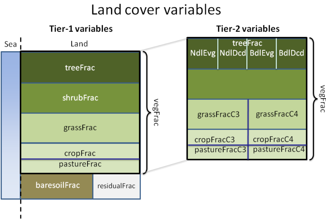
Figure 11: Requested land cover variables. Sea fraction is assume to be fixed, so must be reported under "climatology". Fractions must sum to 1 for every grid cell (including the sea fraction). Fractions are per grid cell, not per land area.
