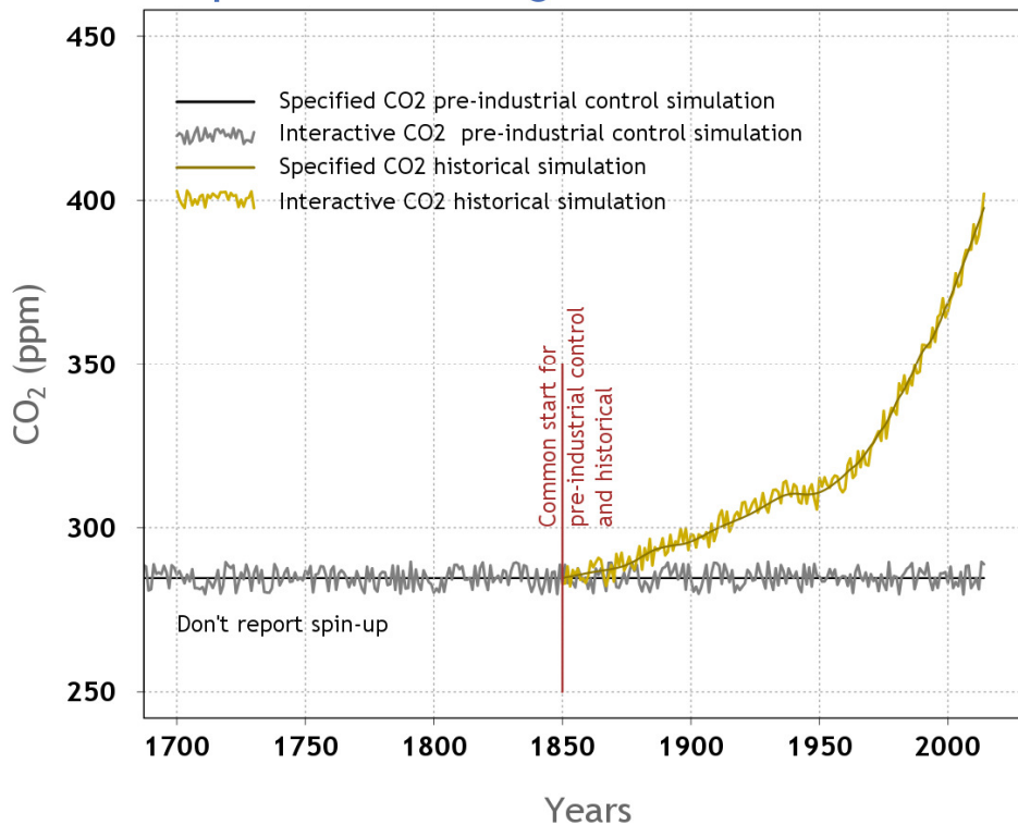
Figure 3. Schematic representation of model spin-up followed by control and historical simulations through 2014. The interactive CO 2 pre-industrial control should ideally have a drift of less than 5 ppm/century.
