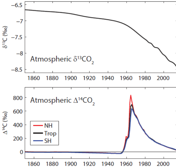
Figure 4. Carbon isotopes in atmospheric \text{CO}_2 for the historical period 1850-2014. Data for \delta^{13}\text{C} is from Law Dome and South Pole (Rubino et al., 2013) and Mauna Loa (Keeling et al., 2001) and includes smoothing of the observations. Data for \Delta^{14}\text{C} is compiled from Levin et al. (2010) and other sources (I. Levin personal communication), following a similar dataset used by Orr et al. (2000).
