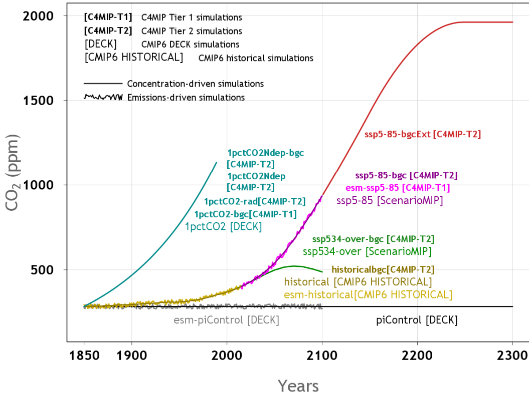
Figure 1: Relation of C4MIP simulations to CMIP6 DECK and historical simulations and the ssp585 and ssp5-34-over future scenario simulation proposed for the ScenarioMIP. Note that at the time of preparing this manuscript the details of the SSP5-3.4-OS-Ext extension to 2300 are not available, hence it could not be included in the figure, but it is still requested as a C4MIP tier-2 simulation.
