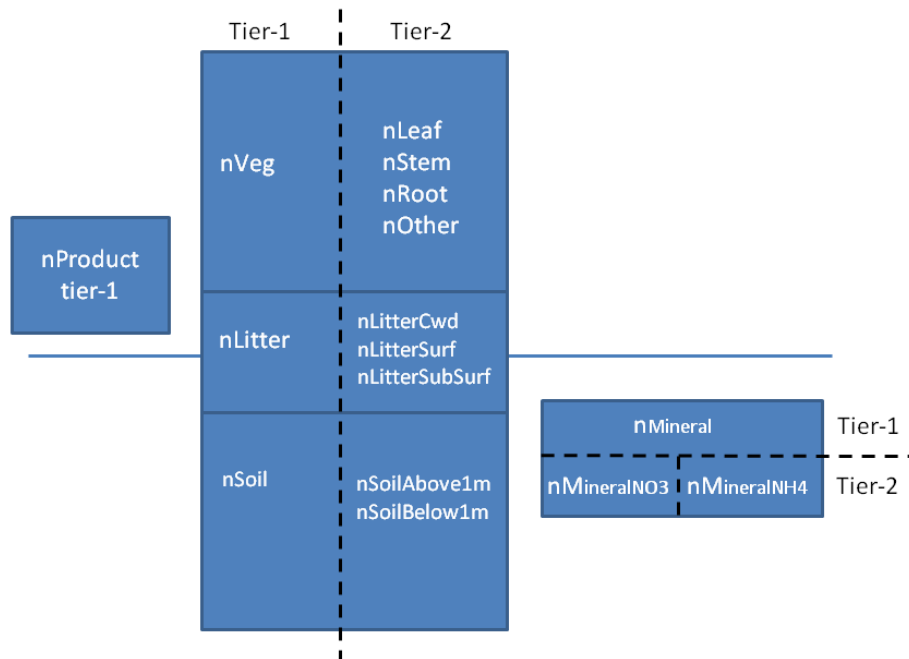
Figure 7: Requested tier-1 and tier-2 variables representing land nitrogen pools.
