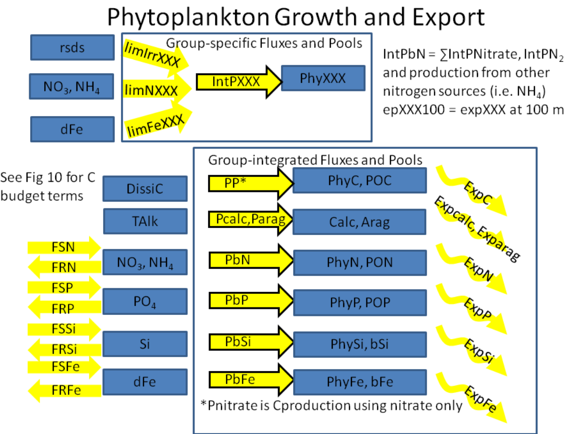
Figure 15: Phytoplankton growth and export variables by phytoplankton group and by associated elemental cycle including external sources and removal. Export refers to the export flux due to sinking.
