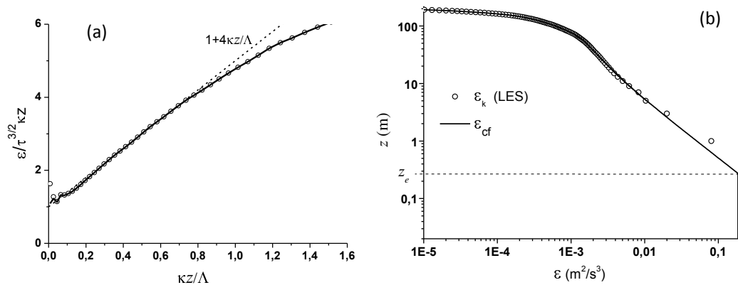
Figure 10. (a) Discrete (LES) nondimensional dissipation \epsilon_{\Delta k} \kappa z_k / |\tau|^{3/2} (circles), corrected values (solid line), universal function (Eq. 44) (dashed straight line). (b) Simulated discrete dissipation \epsilon_{\Delta k} (circles) and corrected dissipation \epsilon_{cf}(z) for LSM (solid line). Dashed horizontal line denotes the height z_e , which was chosen in order to equalize the integral values of the corrected dissipation and the discrete dissipation.
