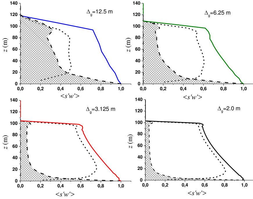
Figure 3. Total F_s^{tot} = \langle \overline{s w} \rangle + \langle \vartheta_3^s \rangle (solid lines), resolved F_s^{res} = \langle \overline{s w} \rangle (short-dashed lines) and "subgrid" F_s^{sbg} = \langle \vartheta_3^s \rangle (long-dashed lines with shading) scalar fluxes in the runs with different grid steps \Delta_g .
