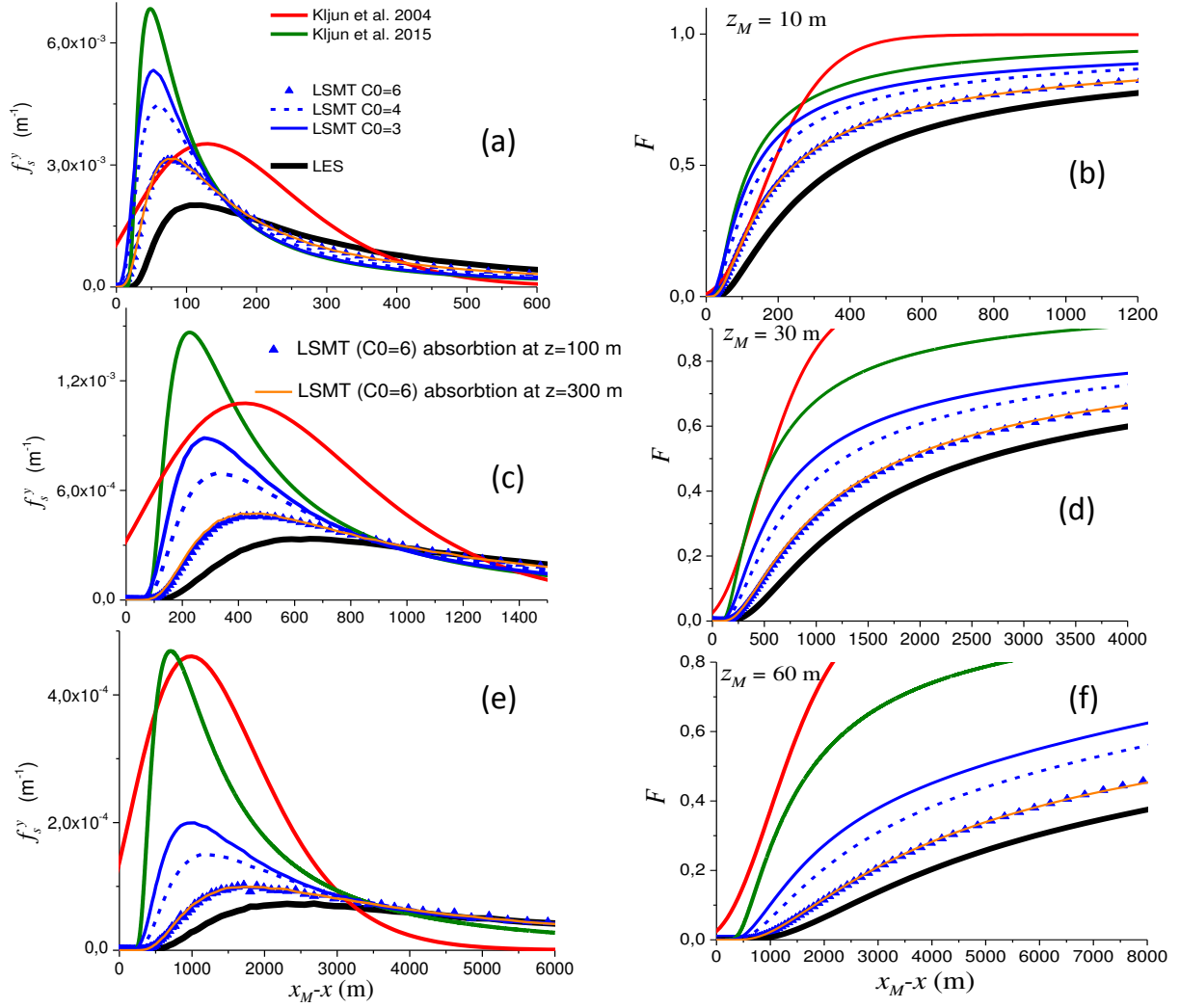
Figure 13. Crosswind-integrated footprints f_s^y (a,c,e) and cumulative footprints F (b,d,f) for sensor height z_M = 10 m (a,b), z_M = 30 m (c,d) and z_M = 60 m (e,f). Solid lines - LES with grid steps \Delta_g = 2.0 m. Triangles - LSMT (Thomson (1987) model), C_0 = 6 , absorption at z=100 m. Orange curves LSMT, C_0 = 6 , absorption at z=300 m. Dashed blue lines - LSMT, C_0 = 4 . Solid blue lines - LSMT, C_0 = 3 . Red lines - parameterisation (Kljun et al., 2004). Green lines - parameterisation (Kljun et al., 2015).
