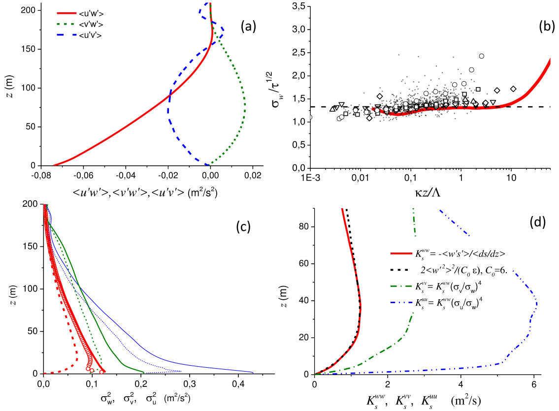
Figure 9. (a) Total momentum fluxes obtained in LES with \Delta_g=2.0 m. (b) Normalized RMS of vertical velocity \tilde{\sigma}_w = \sigma_w/|\tau|^{1/2} depending on a dimensionless parameter z/\Lambda (solid red line - estimation using LES data \sigma_w = (\langle w'^2 \rangle + 2/3 E_{subgr})^{1/2} ; symbols - measurements (Grachev et al., 2013) at different heights). (c) Variances of velocity components (dashed line - resolved fluctuation; solid lines - the final estimation for LSM; bold red lines - vertical component, green curves of medium thickness - crosswind component, blue thin lines - longitudinal component, circles - evaluation of \sigma_w^2 by Eq. (41)). (d) Vertical effective eddy diffusivity K_s^{ww} (red solid line - coefficient calculated by the gradient and flux of scalar; dashed line - estimation of coefficient using Eq. (13) with C_0 = 6 ); estimations of diffusion coefficients in crosswind direction K_s^{vv} (green dash-dot line) and coefficient in longitudinal direction K_s^{uu} (blue dash-dot-dot line).
