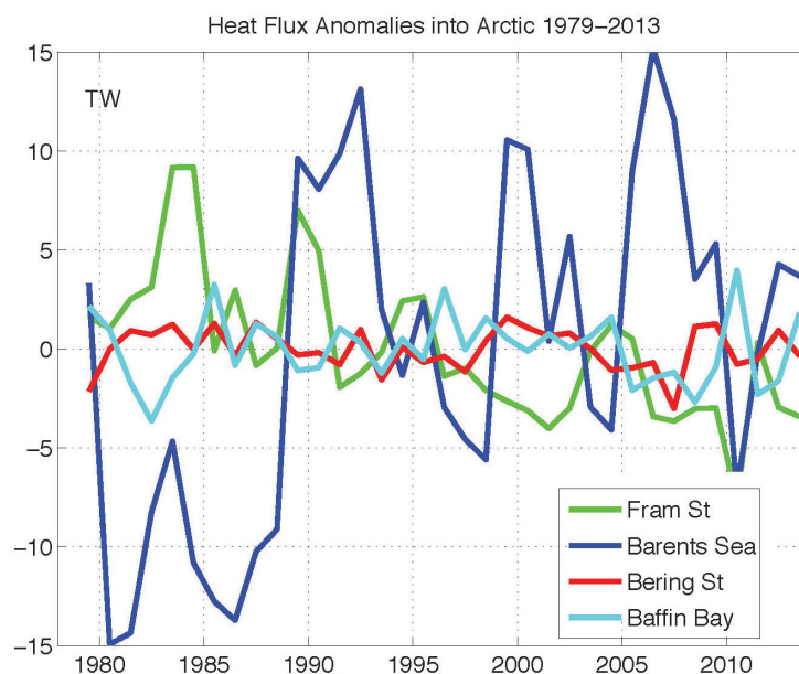
Figure 4. Heat flux anomalies (seasonal cycle removed) across key Arctic Straits as indicated in Fig.2. The units are in TW.
