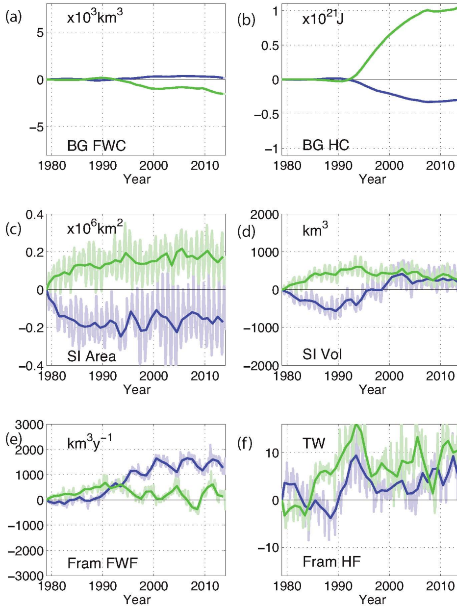
Figure 7. CRFs for the Greenland Sea wind anomaly, blue (+) and green (-). Note that the (+) sign implies a stronger cyclonic forcing. The response to a 4hPa surface pressure anomaly (see Fig.5b) is shown of (a) C_{FWC_{BG}}^{WGS} , the FWC of the BG (b) C_{HC_{BG}}^{WGS} , HC of the BG (c) C_{SIA}^{WGS} , SI area (d) C_{SIV}^{WGS} , SI volume (e) C_{FWF_{Fram}}^{WGS} , FWF through the Fram Strait and (f) C_{HF_{Fram}}^{WGS} , the HF through the Fram Strait.
