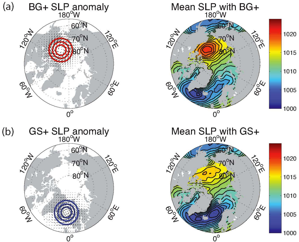
Figure 5. (a) (left) Idealized sea-level pressure anomaly of 4hPa and associated winds constructed for the Beaufort Gyre (BG). Note the BG(+) corresponds to anomalously high pressure. (right) BG(+) SLP anomaly added to the NCEP 1981-2010 SLP climatology. (b) (left) Idealized sea-level pressure anomaly of 4hPa and associated winds constructed for the Greenland Sea (GS). Note the GS(+) corresponds to anomalously low pressure over the GS. (right) GS SLP anomaly added to the 1981—2010 SLP climatology.
