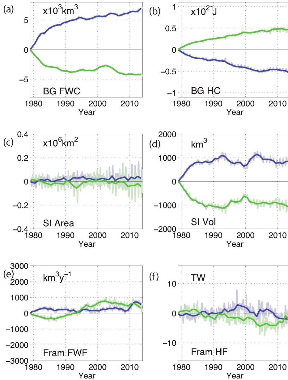
Figure 6. CRFs for the Beaufort Gyre wind anomaly, blue (+) and green (-). Note that the (+) sign implies a stronger anti-cyclonic forcing. The response to a 4HPa surface pressure anomaly (see Fig.5a) is shown of (a) C_{FWC_{BG}}^{W_{BG}} , the FWC of the BG (b) C_{HC_{BG}}^{W_{BG}} , HC of the BG (c) C_{SIA}^{W_{BG}} , SI area (d) C_{SIV}^{W_{BG}} , SI volume (e) C_{FWF_{Fram}}^{W_{BG}} , FWF through the Fram Strait and (f) C_{HF_{Fram}}^{W_{BG}} , the HF through the Fram Strait.
