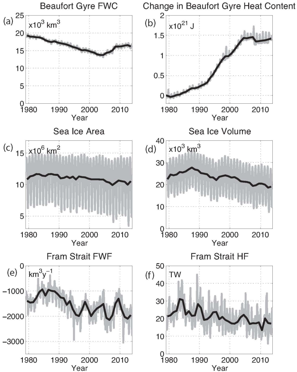
Figure 3. Time-series of (a) fresh water content (FWC) and (b) heat content (HC) of the BG, (c) sea-ice area and (d) sea-ice volume over the Arctic, (e) fresh water flux (FWF, negative values imply a flux out of the Arctic) and (f) heat flux through Fram Strait (HF, positive values indicate a flux in to the Arctic). The thick black line plots annual-mean values, the grey line tracks monthly-means.
