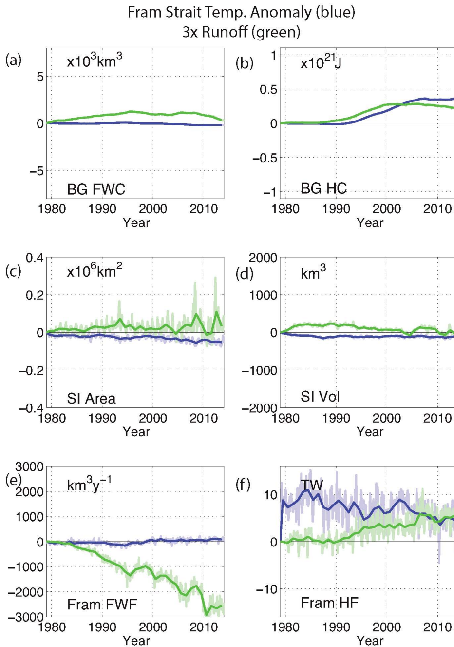
Figure 8. CRFs in response to an impulsive 3 x Runoff (green lines) and Fram Strait T (+2C) anomaly (blue lines): (a) the FWC of the BG (b) HC of the BG (c) SI area (d) SI volume (e) FWF through the Fram Strait and (f) the HF through the Fram Strait.
