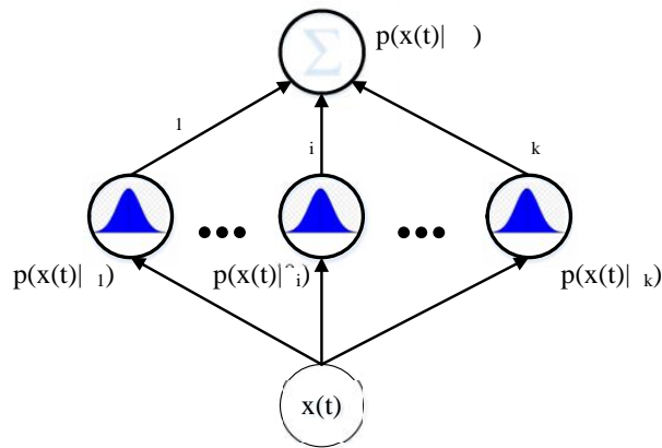
Figure 3 Structure of Gaussian Mixture Model (GMM)
