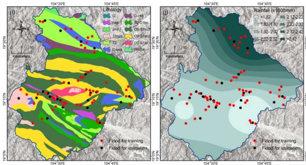
155 Figure 2 (Cont.) Flood influencing factors: (e) Stream power index, (f) Distance to river, (g) Stream density, (h) Normalized Difference Vegetation Index, (i) Lithology, (j) Rainfall
