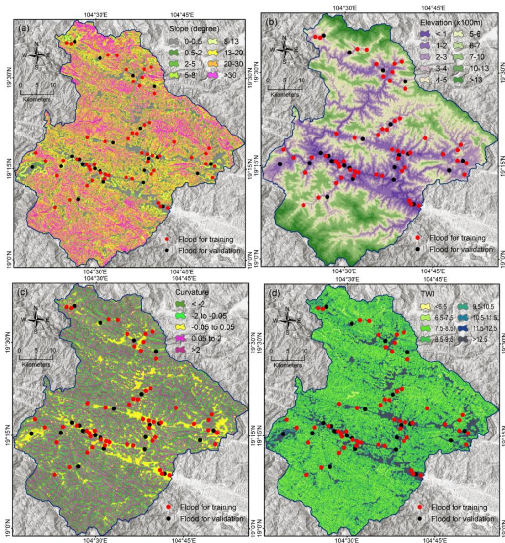
Figure 2 Flood influencing factors: (a) Slope, (b) Elevation, (c) Curvature, (d) Topographic wetness index
