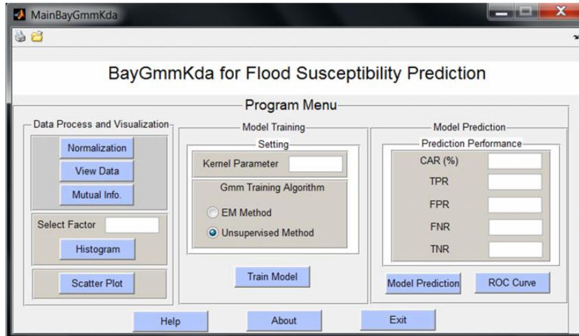
Figure 6 Main Menu of BayGmmKda
