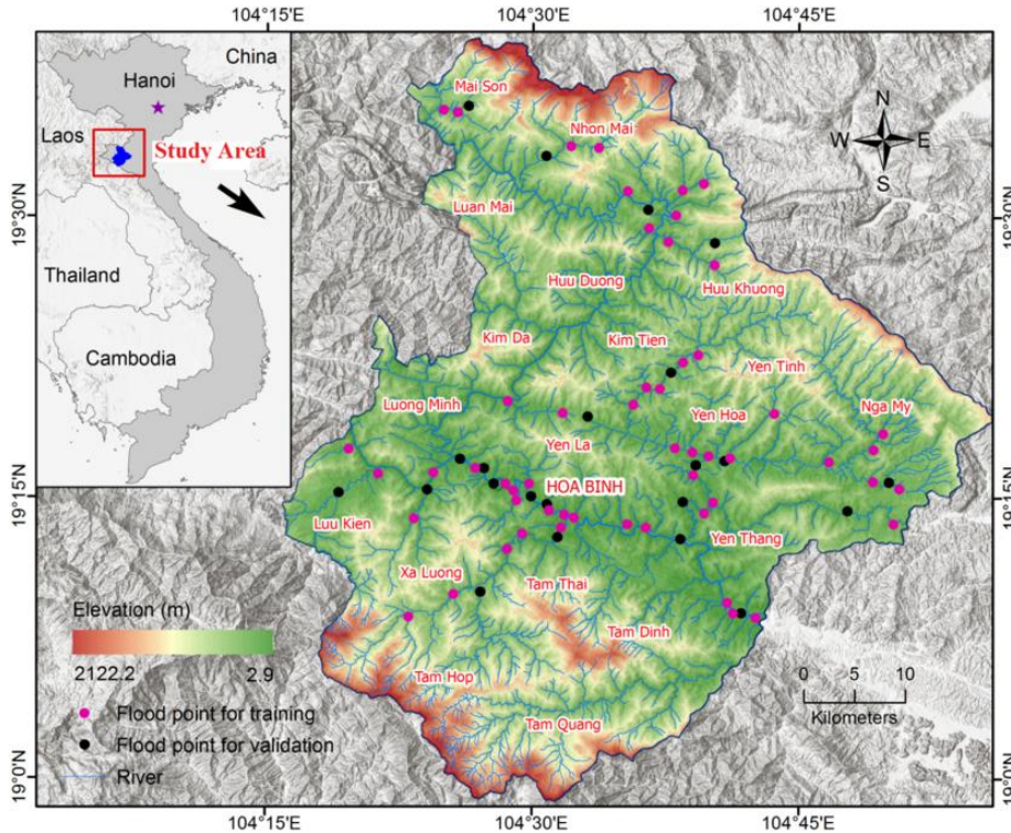
Figure 1 Tuong Duong district (Central Vietnam)
