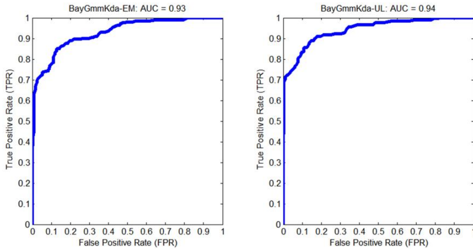
Figure 9 ROC plots of the proposed BayGmmKda
