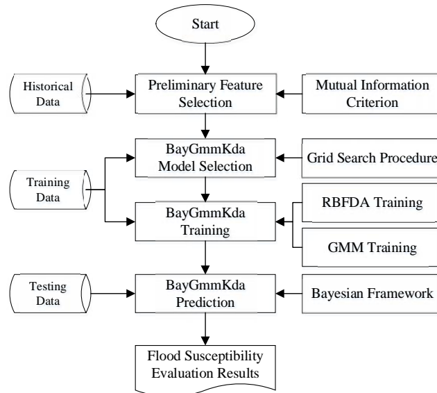
Figure 5 The proposed BayGmmKda
