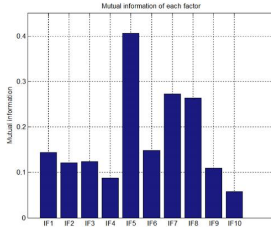
Figure 7 Mutual information of flood conditioning factors
