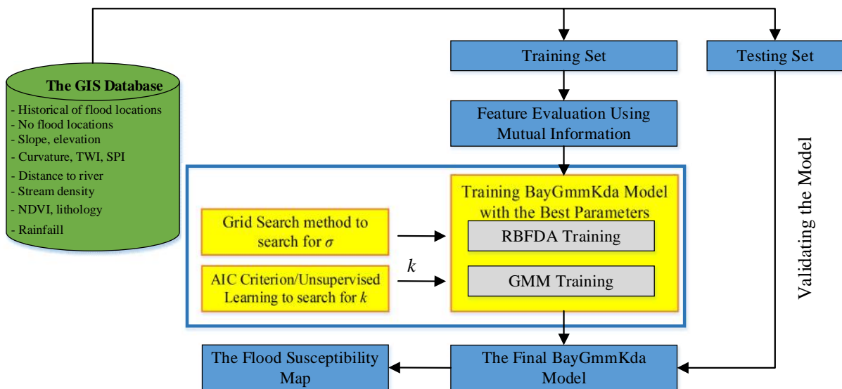
Figure 6 The proposed BayGmmKda
