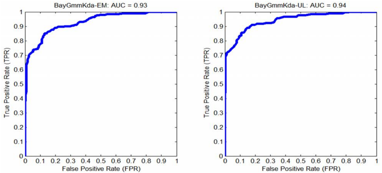
Figure 9 ROC plots of the proposed BayGmmKda
