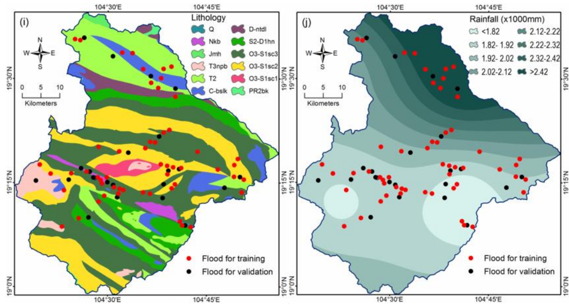
Figure 2 (Cont.) (i) Lithology, (j) Rainfall
