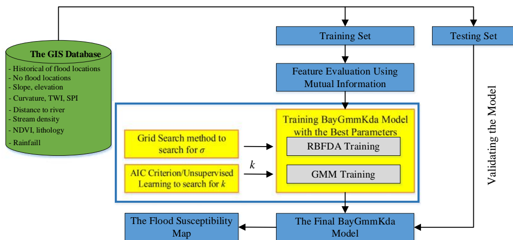
Figure 6 The proposed BayGmmKda
