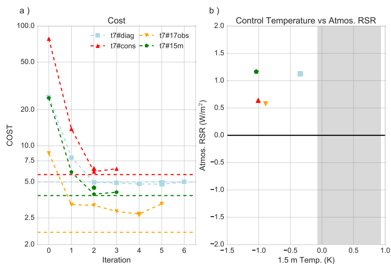
Figure 10. a) Cost as function of iteration for four trial 7-parameter cases (lines and symbols). Also shown are the cost functions for the standard model for each case (coloured horizontal lines) with the colour corresponding to the trial case. Large symbol for each trial case show cost from independent atmospheric simulation with other details as Fig. 1. b) Scatter plot (symbols as a) of optimal minus standard configurations for 2000-2010 mean RSR from atmospheric only simulations against the coupled Control mean for years 10-19 of 1.5 m temperature. Vertical grey region show estimates of the difference between pre-industrial global-average air temperatures and the standard configuration; configurations in this region are "good".
