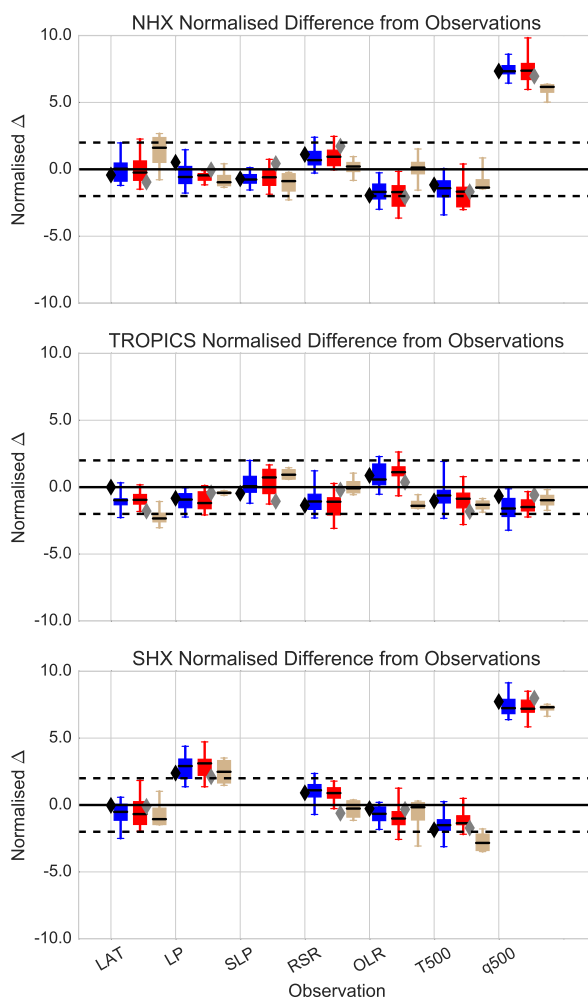
Figure 5. As Fig. 3 except shown are differences between simulated, from 2-member ensemble, and observed change between 2005-2010 and 2000-2005. All values are standardised by 3\sigma internal variability computed from the 100 member 2000-2005 HadAM3 ensemble.
