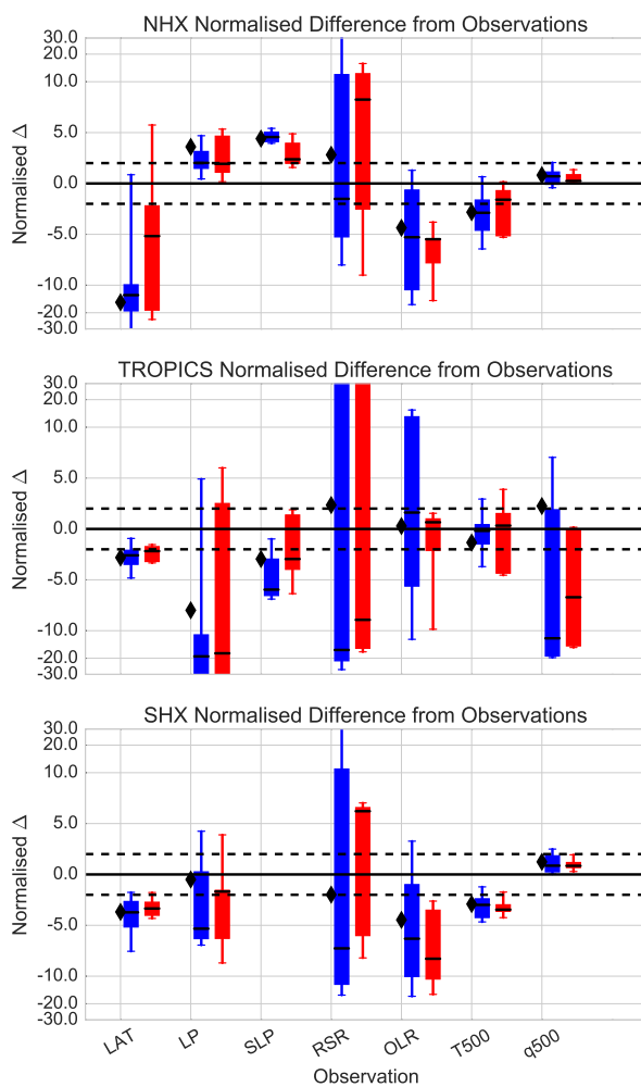
Figure 4. As Fig. 3 except shown are initial extreme random parameter choices for 7-(red) and 14-parameter (blue) cases.
