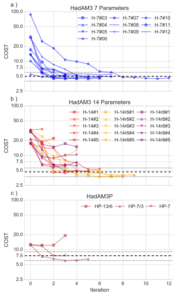
Figure 1. Minimum cost function for "line-search" component of algorithm (y-axis) versus iteration number (x-axis) for HadAM3 7-parameter (a), HadAM3 14-parameter (b) and HadAM3P (c) optimisations. Iteration 0 is the cost function for the initial parameter values. The y-axis uses a logarithmic scale. In each subplot the dashed black line show the cost function for the standard model while the dotted lines show the \pm 20\% ranges on this showing perturbed models comparable with the standard configuration. Coloured lines and symbols use the key shown in each sub-plot. For plots b) & c) labels with rP rand had P rand random parameters perturbed on each iteration.
