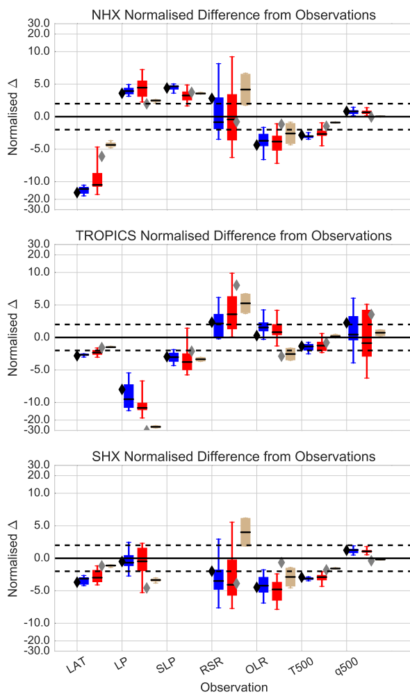
Figure 3. Normalised simulated minus observed distributions (y-axis) for 7 (blue) and 14-parameter (red) cases. Top panel is northern hemisphere extra-tropics, middle tropics and lower southern hemisphere extra-tropics. Boxes and whiskers as Fig. 2, with observations on x-axis. Also shown are the optimised HadAM3P cases (tan boxes/lines) and the standard HadAM3 (black diamonds) and HadAM3P (grey diamonds) values. All differences are normalised by the square root of the diagonal elements of C . The dashed lines show \pm 2 . The scale is linear between 5 and -5 and logarithmic outside that range.
