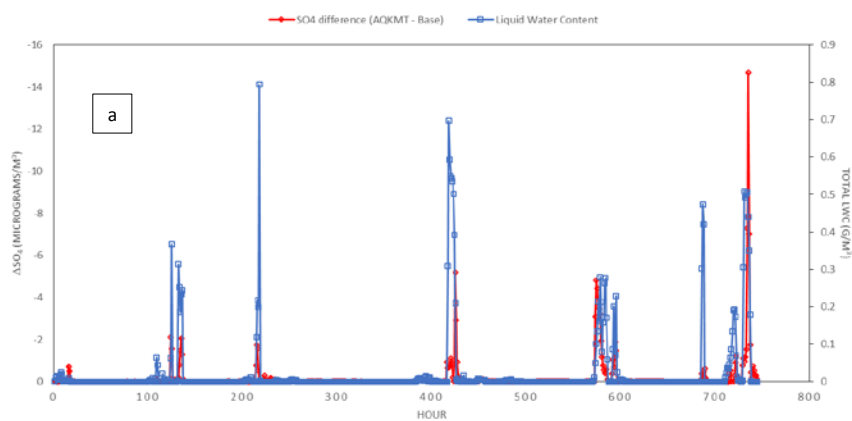
TIME SERIES OF LWC AND \Delta\text{SO}_4\text{IJ} (AQKMT-BASE) AT CELL WITH MAX HOURLY DIFFERENCE AT THE SURFACE FOR JULY 2011 (183,213)
