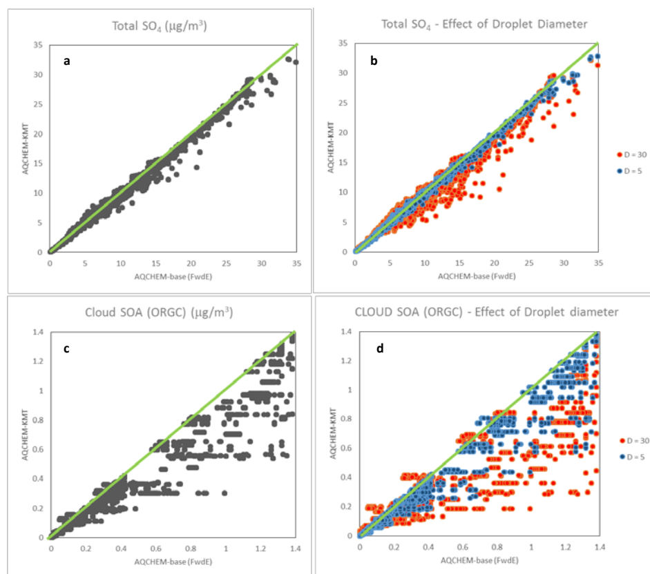
5 Figure 2: AQCHEM-KMT vs. standard AQCHEM predictions for (a) total SO 4 2- (sum over all modes) and (c) SOA from cloud processing of carbonyls (ORGC) at default droplet diameter of 16 μm as well as at 5 and 30 μm for (b) total SO 4 2- and (d) ORGC.
